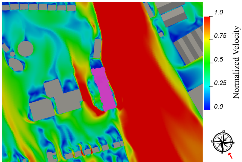
Figure 8.6: Flow Velocity Results at 1.5m above the ground - Wind Direction: 150°
