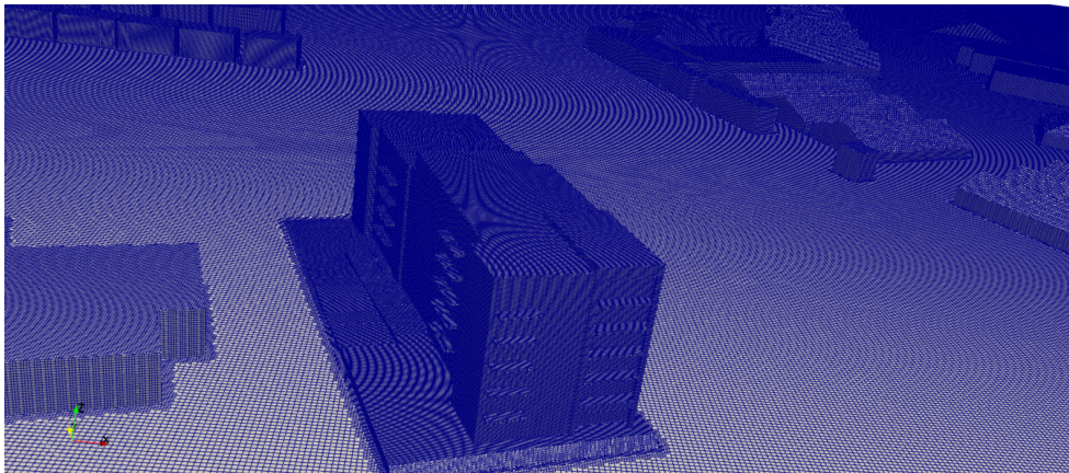
Figure 4.3: Computational Mesh of Proposed Part 8 Residential
