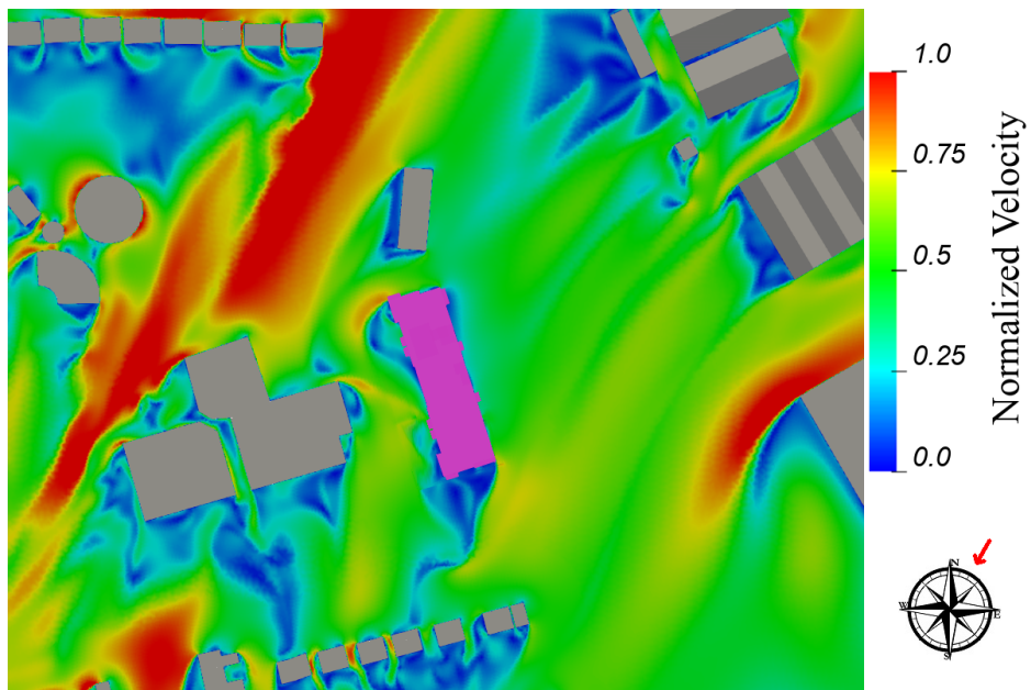
Figure 8.2: Flow Velocity Results at 1.5m above the ground - Wind Direction: 30°
