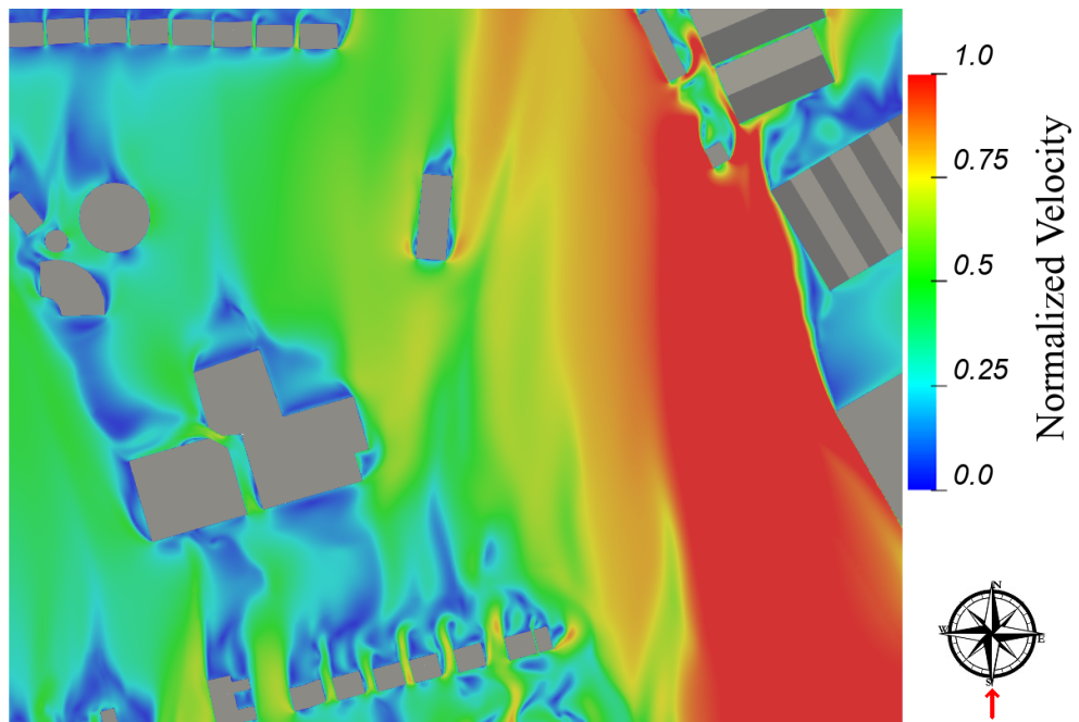
Figure 7.7: Ground Floor Level - Flow Velocity Results at Z=1.5m above the ground - Wind Direction: 180°
