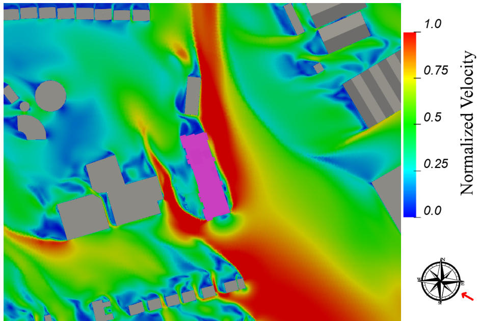
Figure 8.5: Flow Velocity Results at 1.5m above the ground - Wind Direction: 120°
