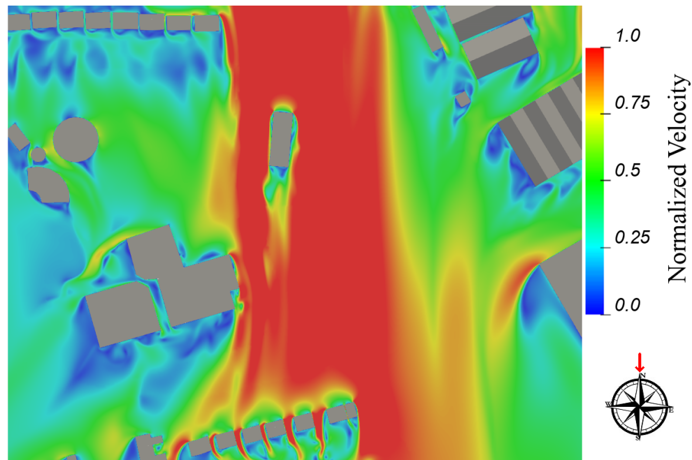
Figure 7.1: Ground Floor Level - Flow Velocity Results at Z=1.5\text{m} above the ground - Wind Direction: 0^\circ
