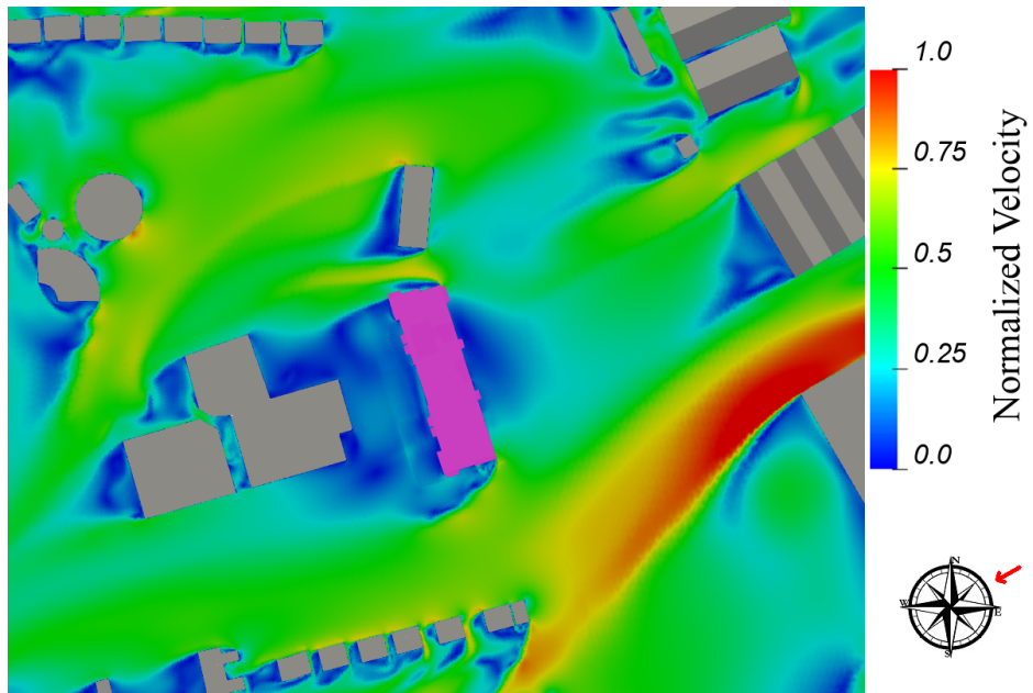
Figure 8.3: Flow Velocity Results at 1.5m above the ground - Wind Direction: 60°
