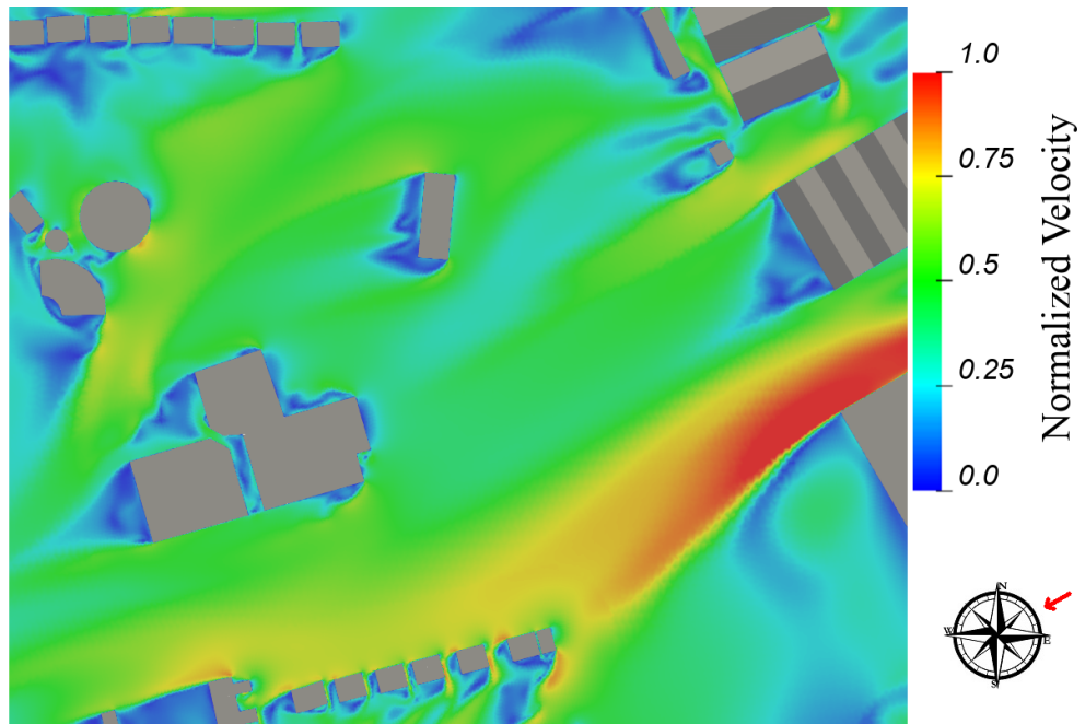
Figure 7.3: Ground Floor Level - Flow Velocity Results at Z=1.5m above the ground - Wind Direction: 60°
