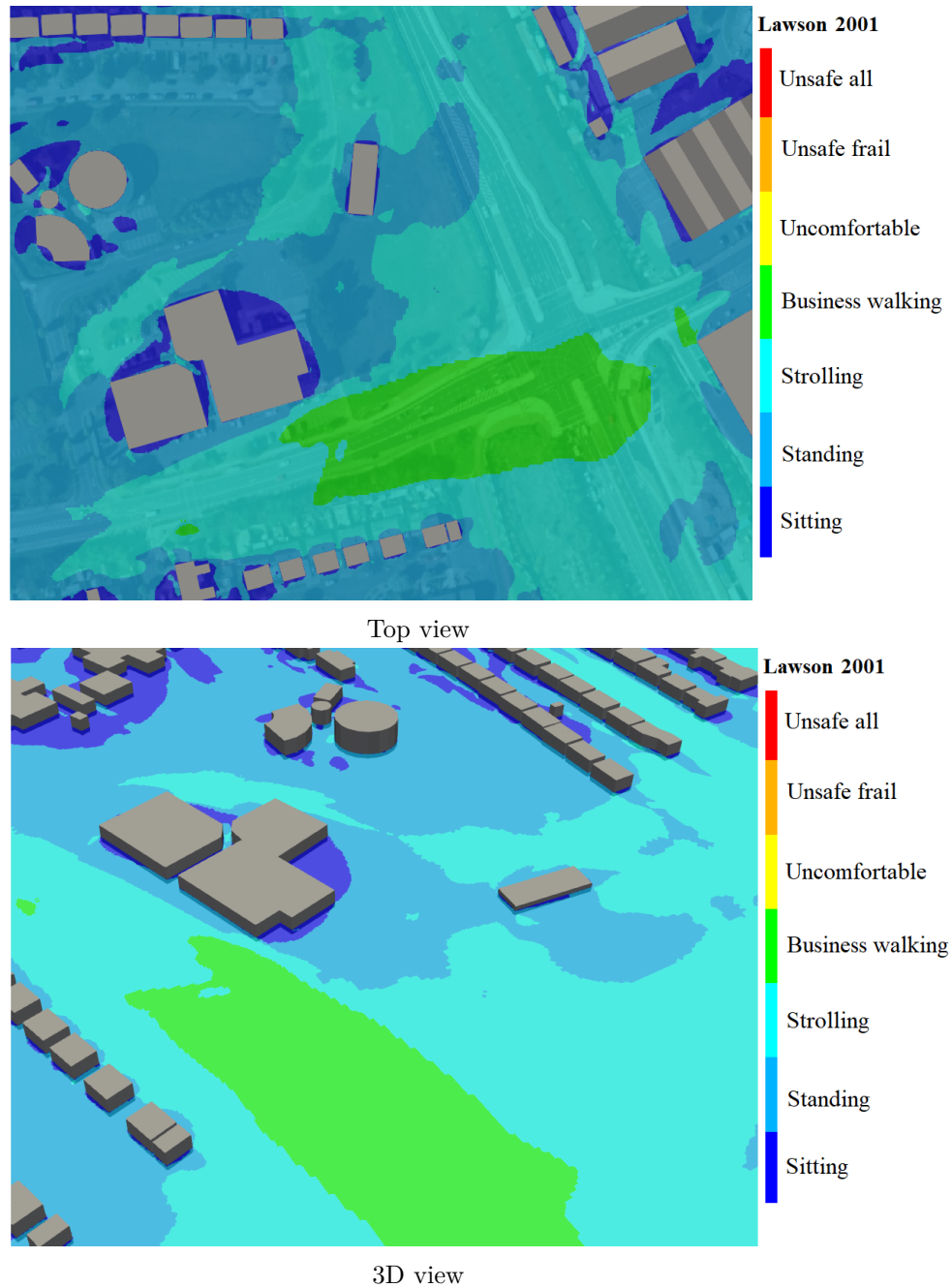
Figure 7.13: Ground Floor - Lawson Discomfort Map - Baseline scenario
