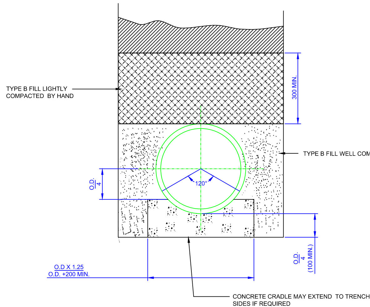
CLASS A BEDDING
