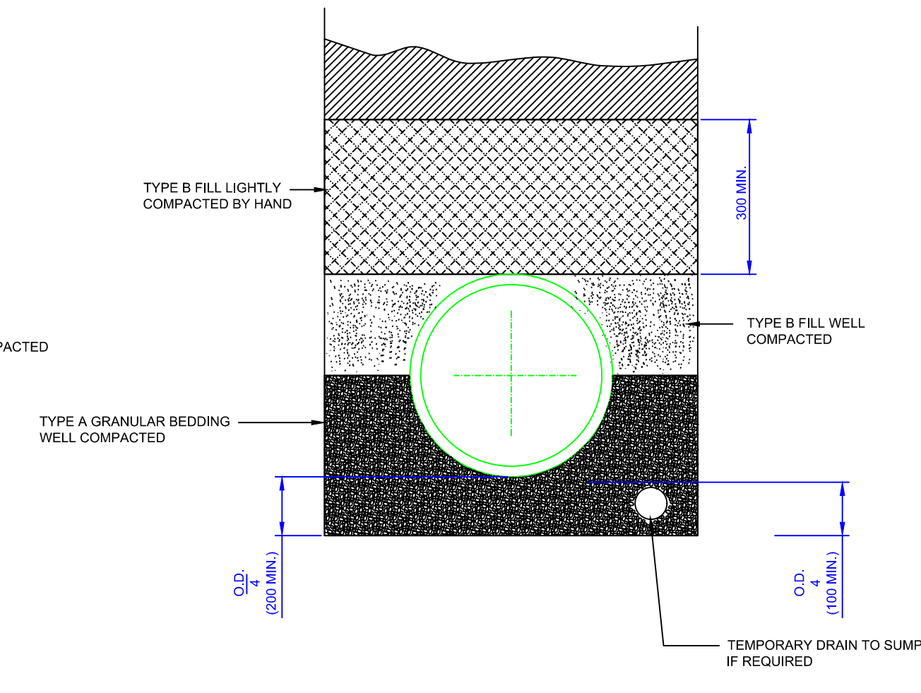
CLASS B BEDDING
