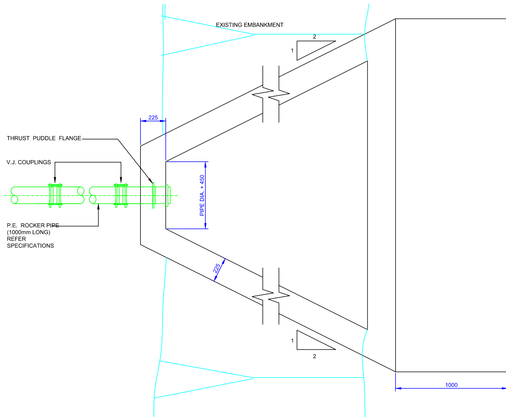
PLAN OUTFALL STRUCTURE
