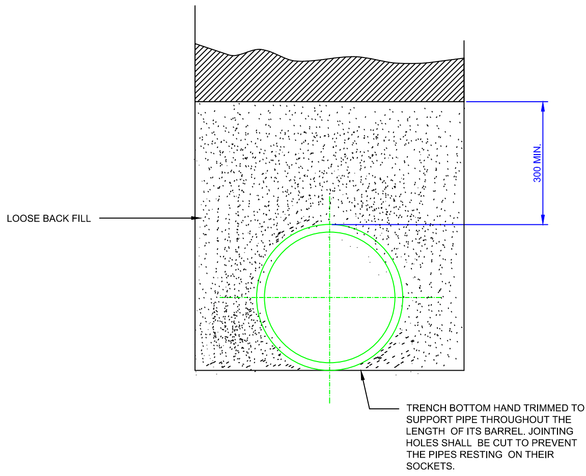
CLASS D BEDDING
