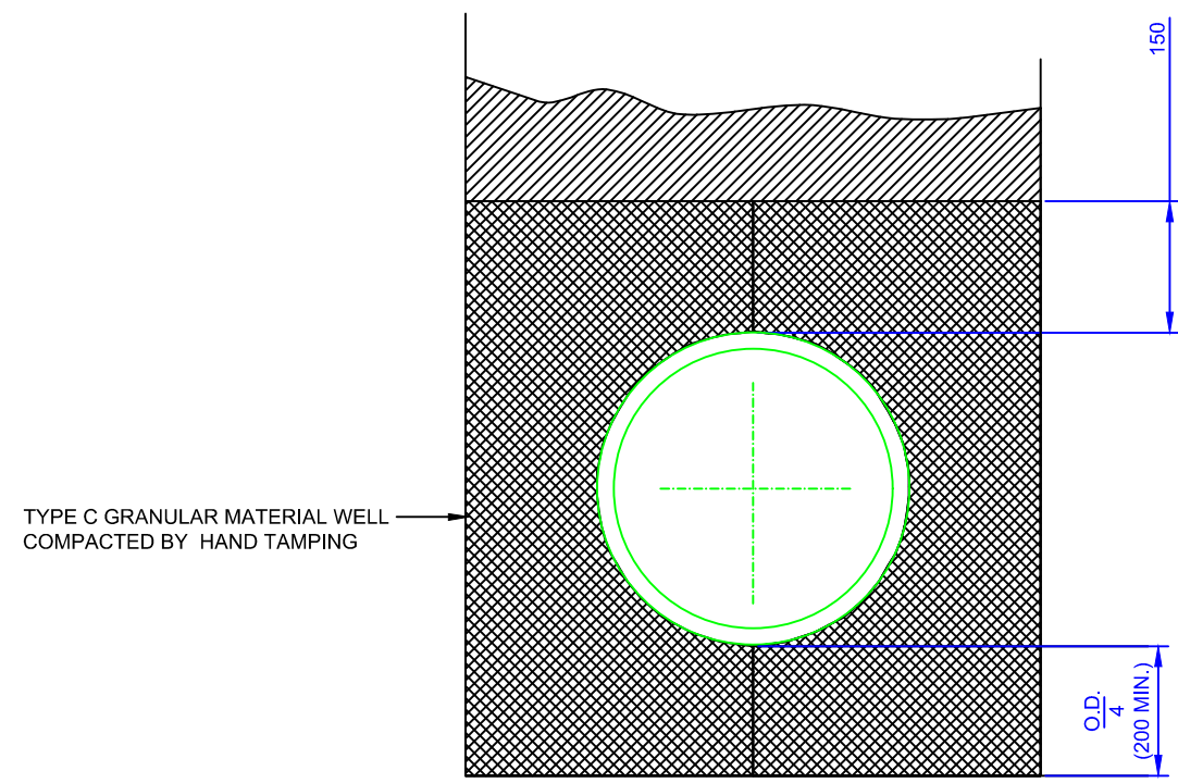
CLASS B BEDDING
