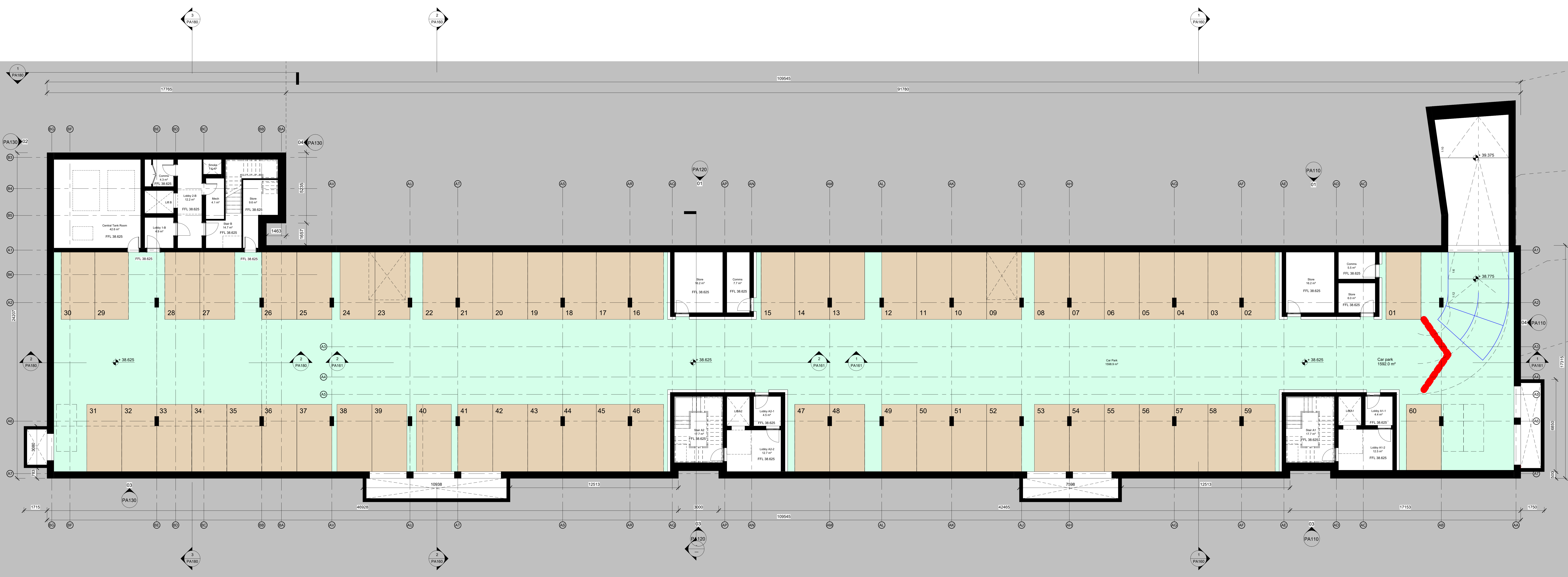
1 Apartment Blocks A1, A2, B - Plan - Level -1 1:100
