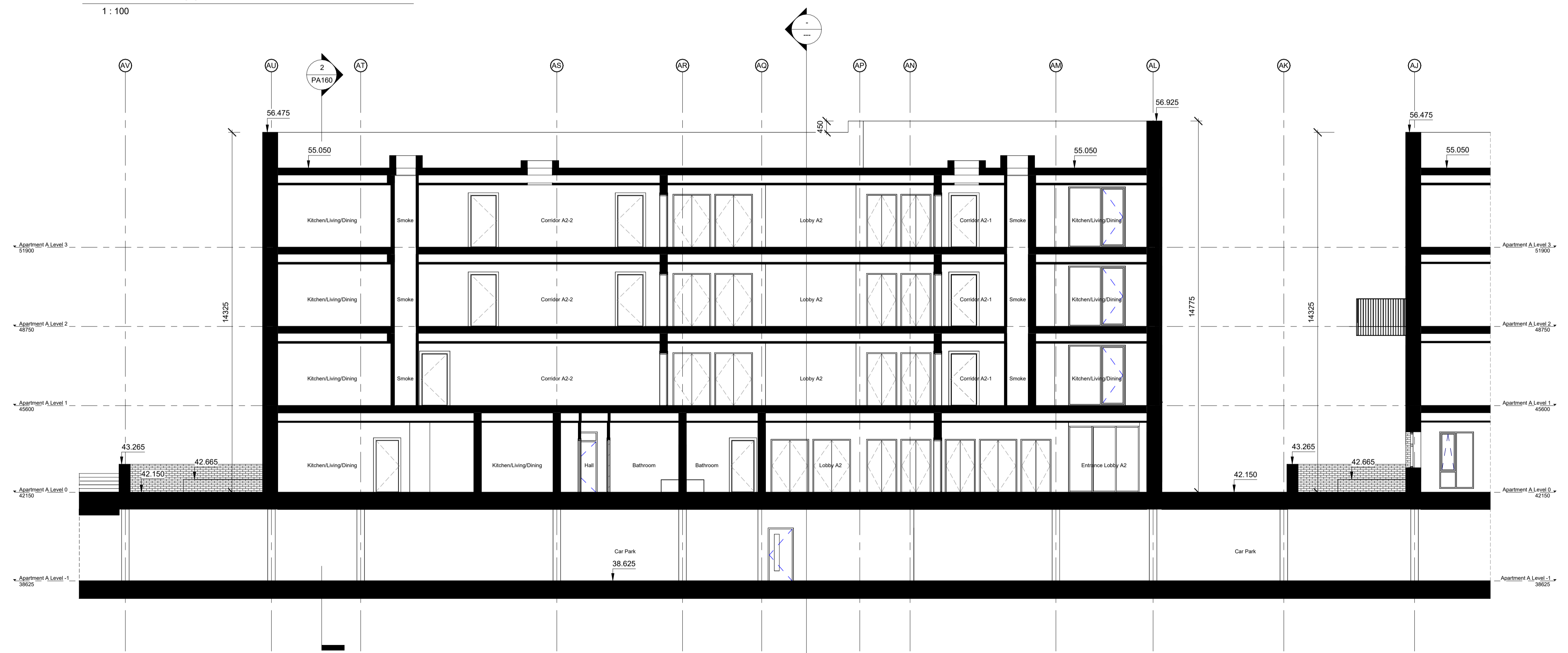
2 Block A - Section 4-4 1:100
