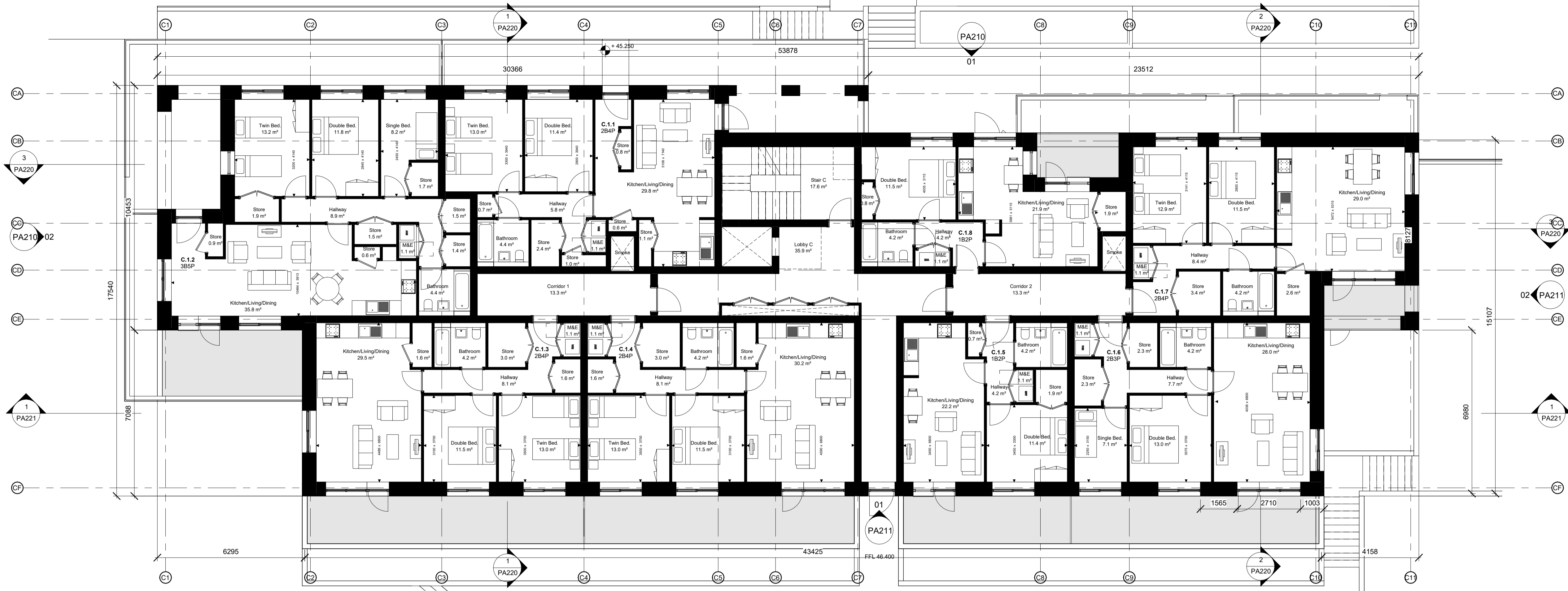
2 Apartment C _ Level 01 1 : 100
