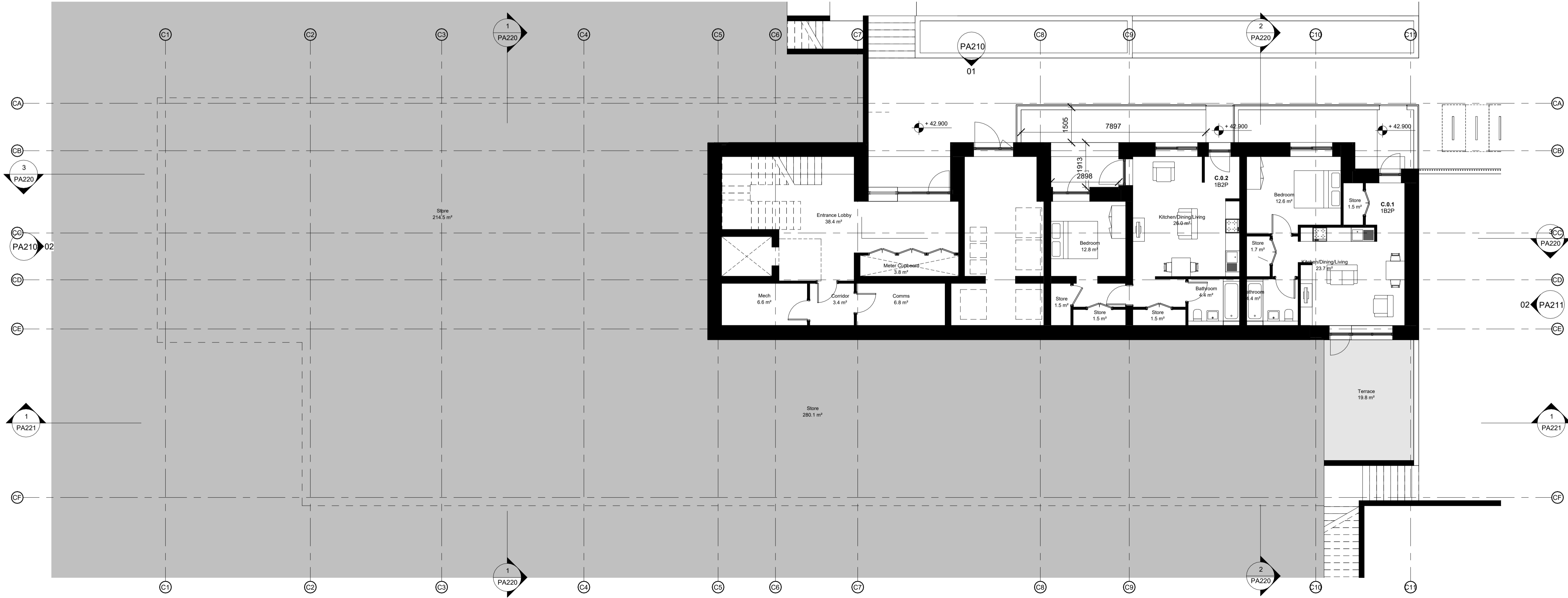
1 Apartment C _ Level 00 1 : 100
