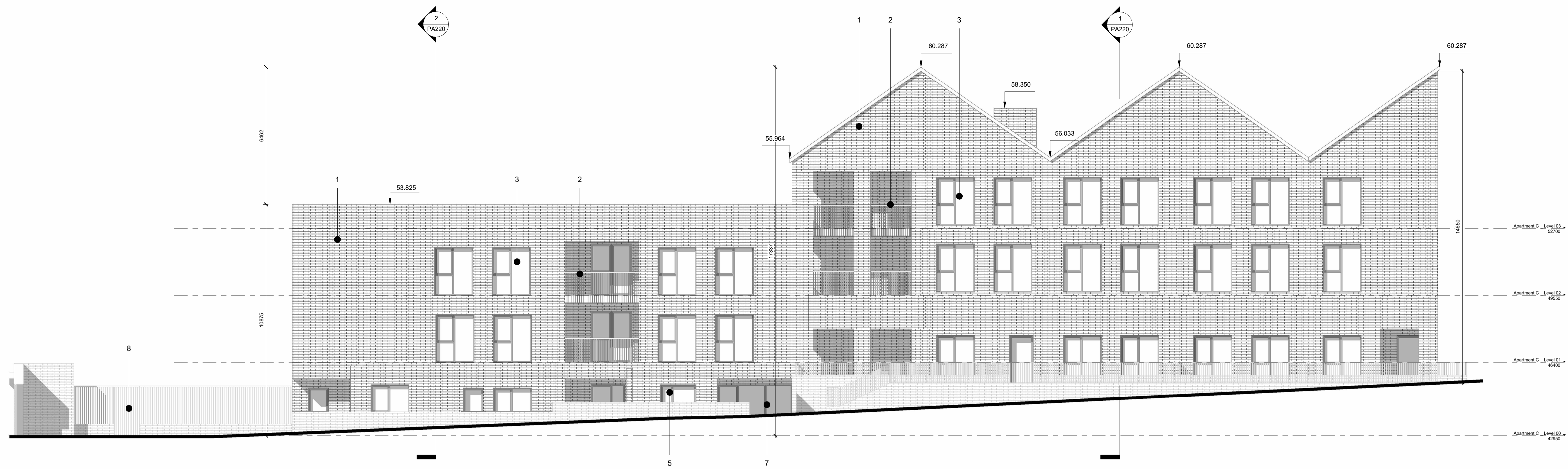
01 Block C - North Elevation 1 : 100
