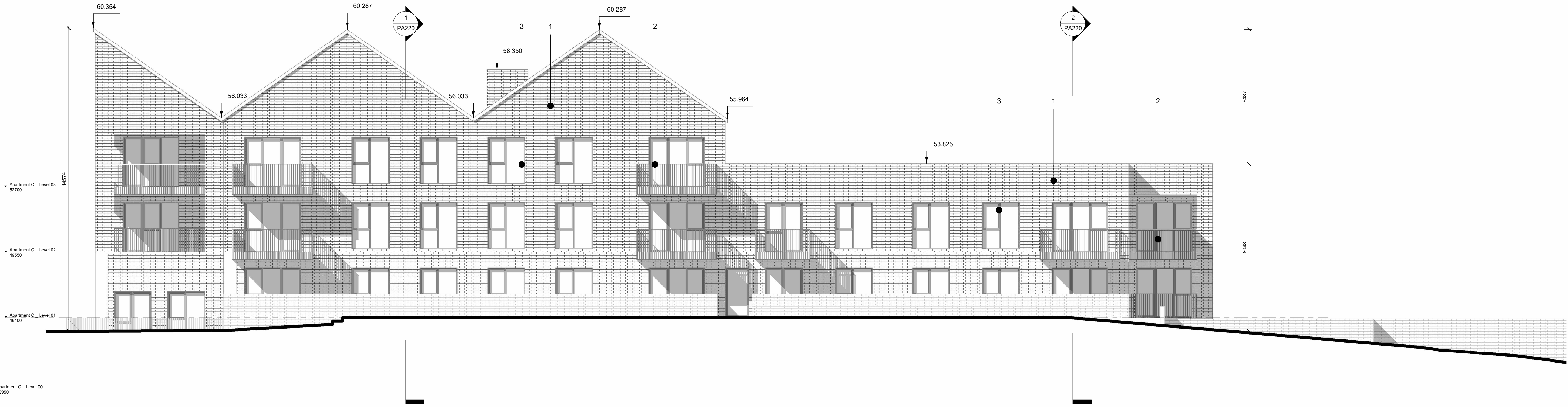
01 Block C - South Elevation 1 : 100
