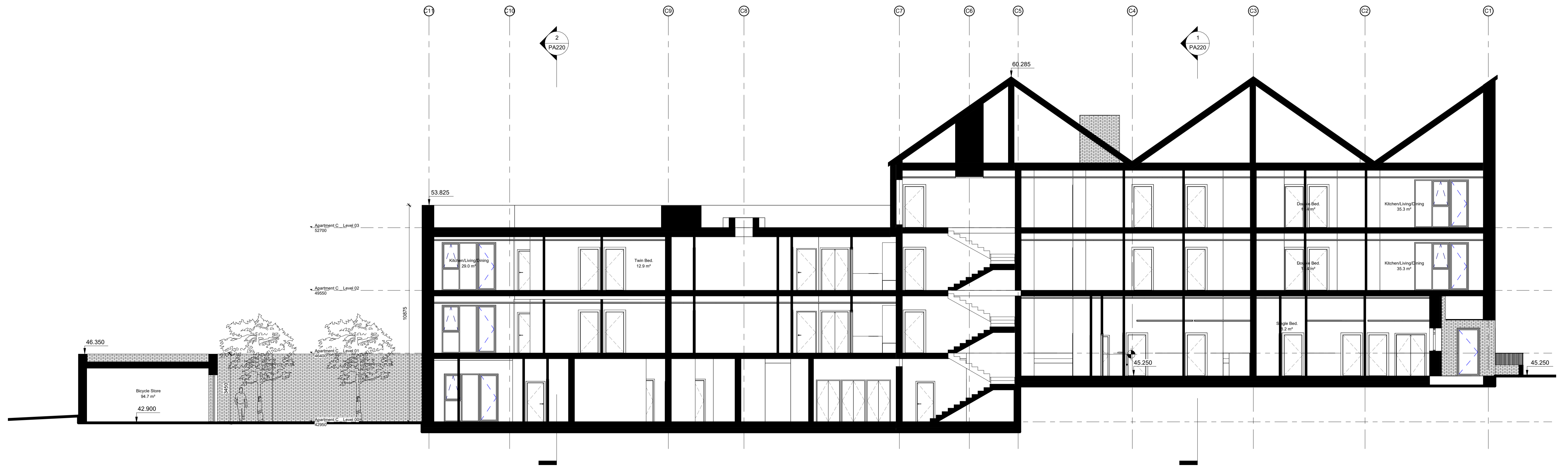
3 Block C - Section 3-3 1 : 100
