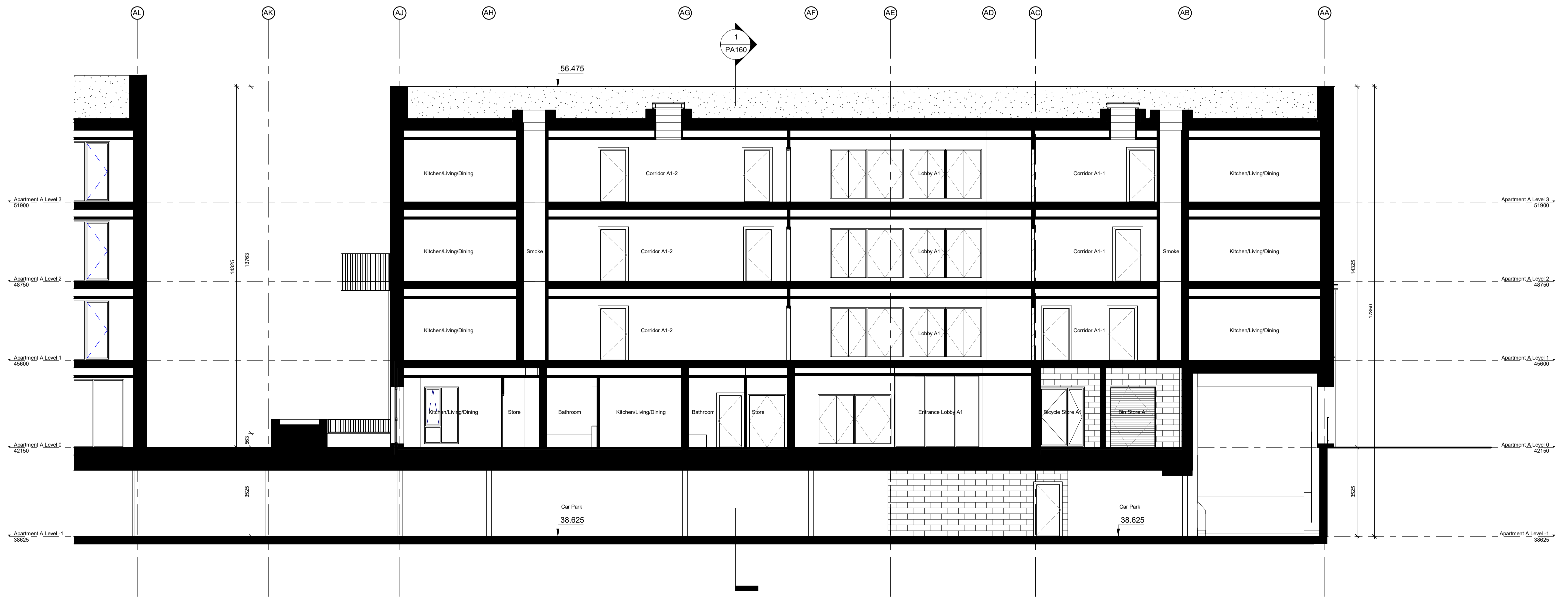
2 Block A - Section 3-3 1 : 100
