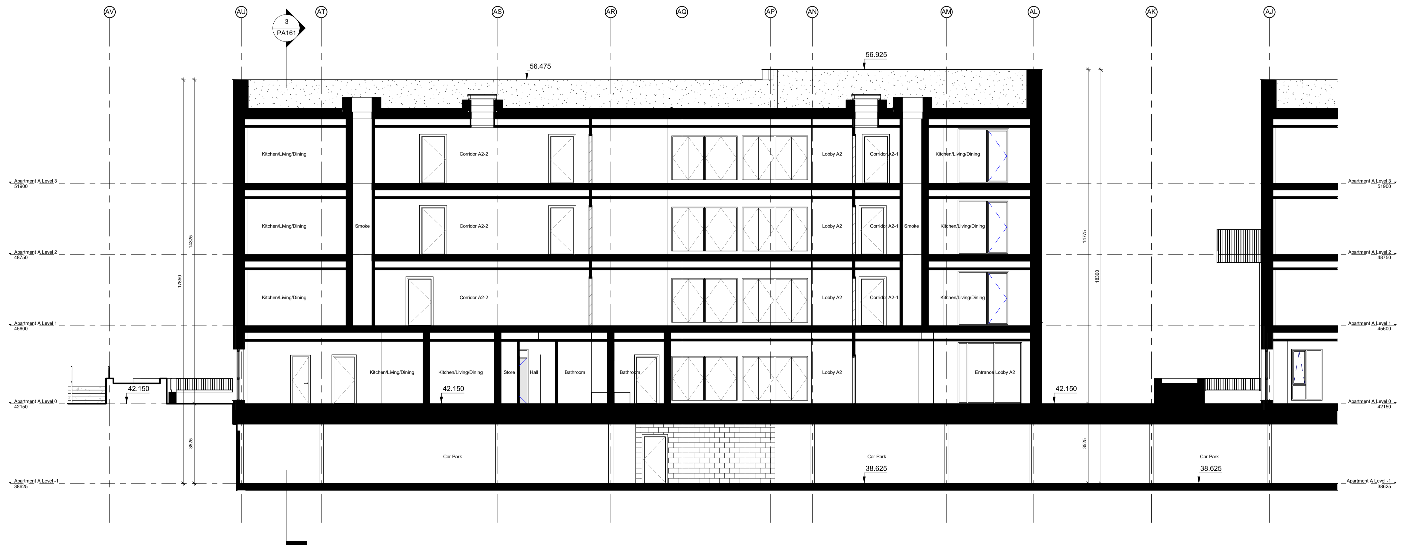
2 Block A - Section 4-4 1 : 100
