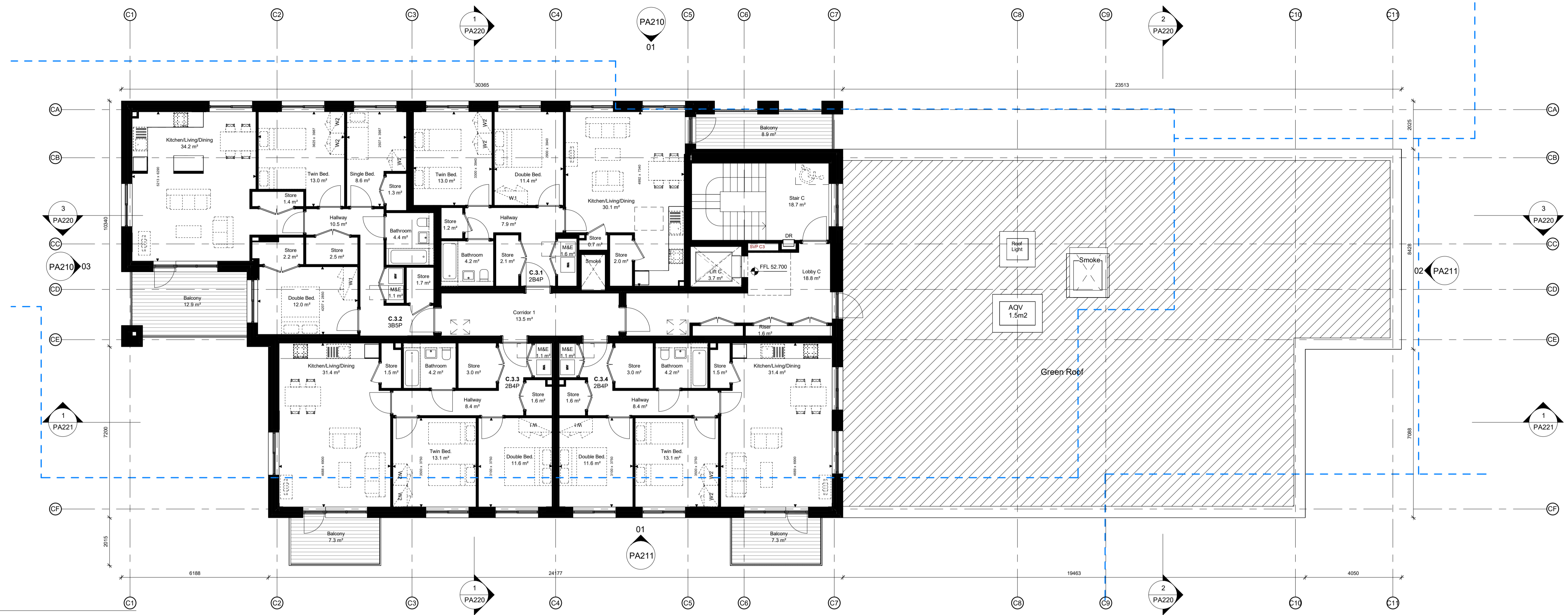
2 Apartment C_Level 03 1: 100
