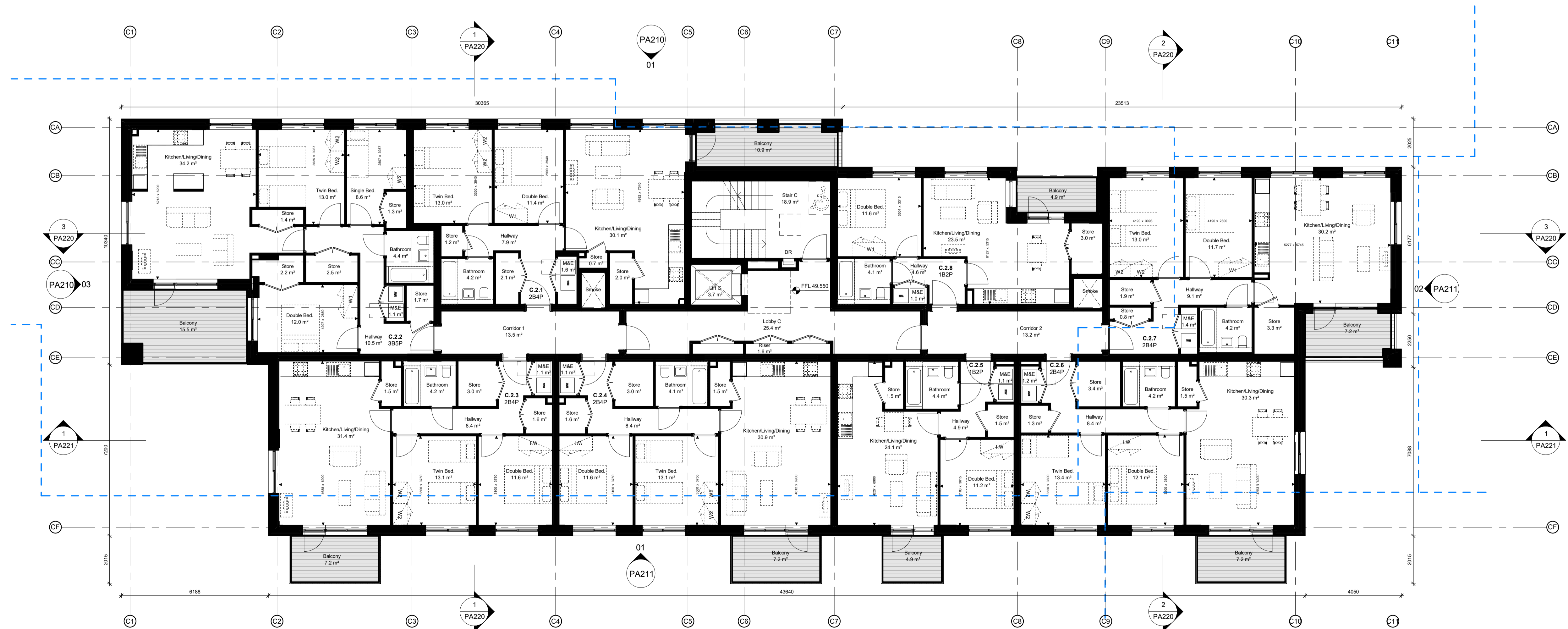
1 Apartment C_Level 02 1: 100
