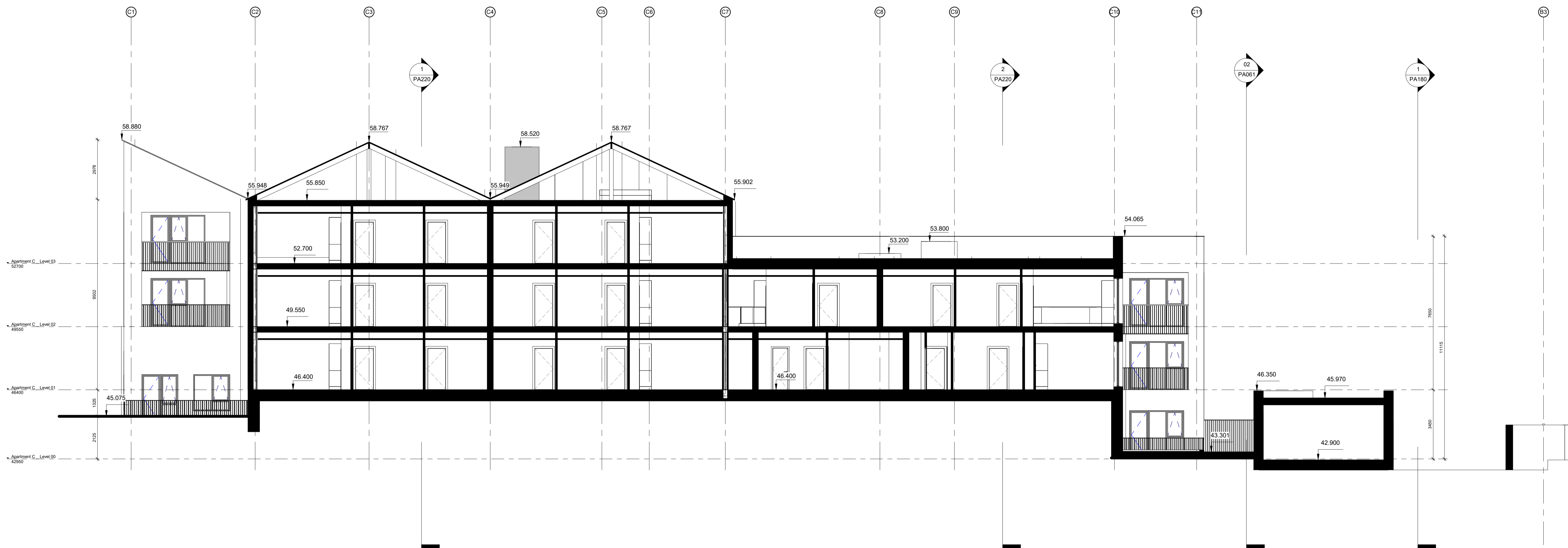
1 Block C - Section 4-4 1 : 100
