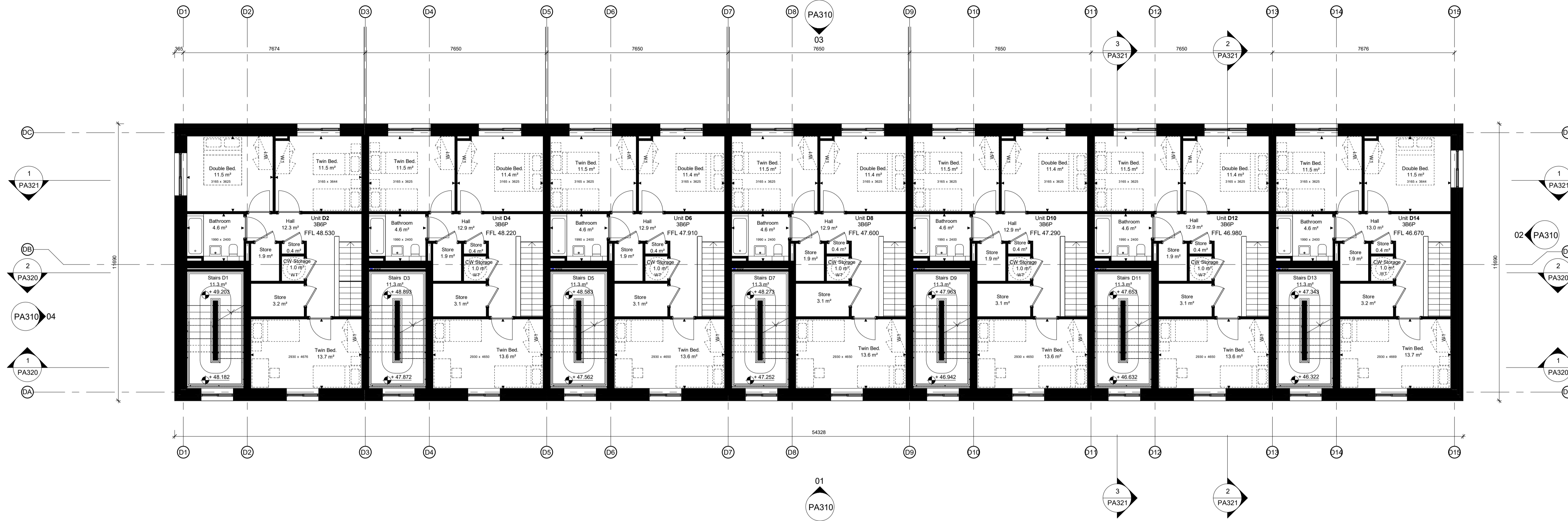
2 Block D_Level 01 1:100
