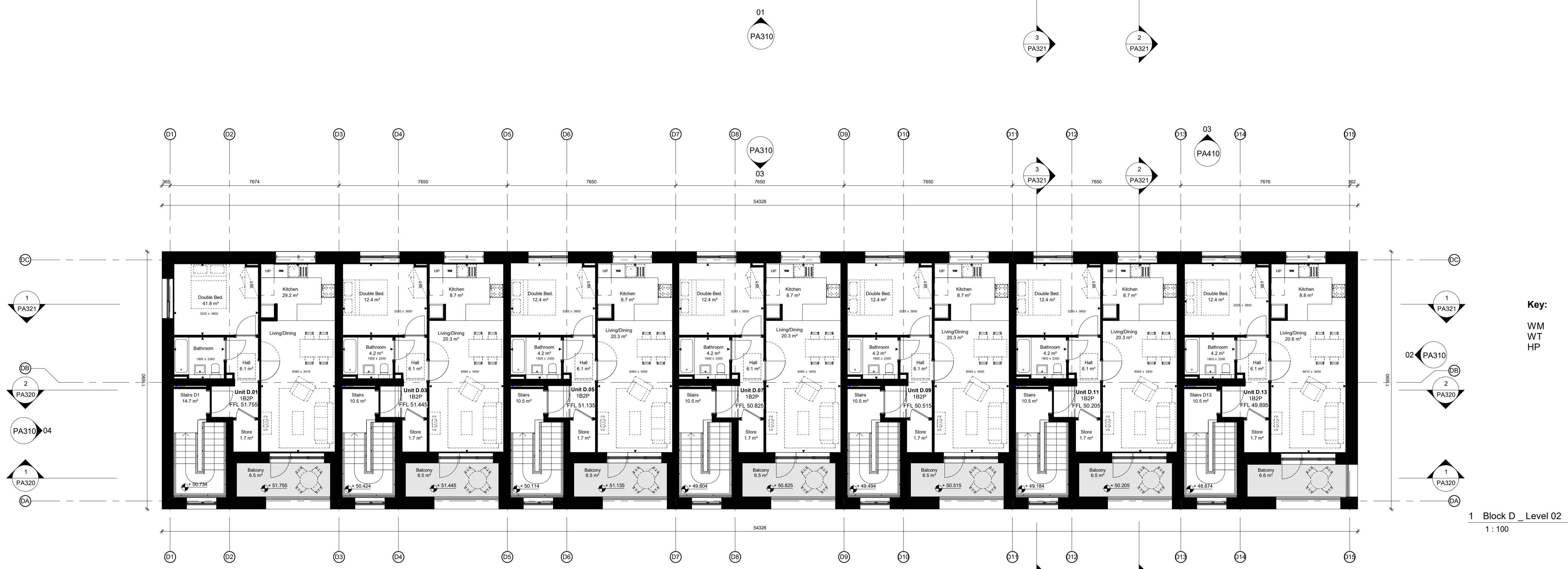
2 Block D_Level 03 1:100
