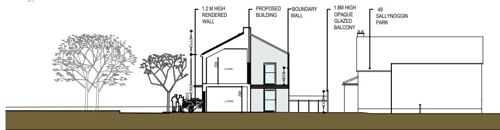
SECTION A - A 1:200
