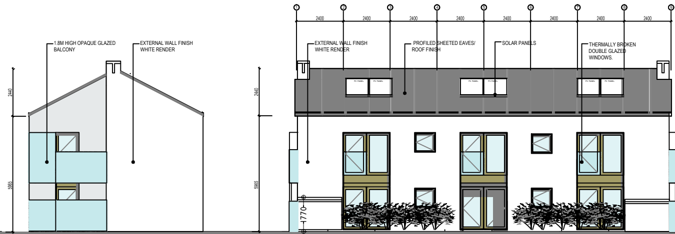
WEST ELEVATION 1:100
