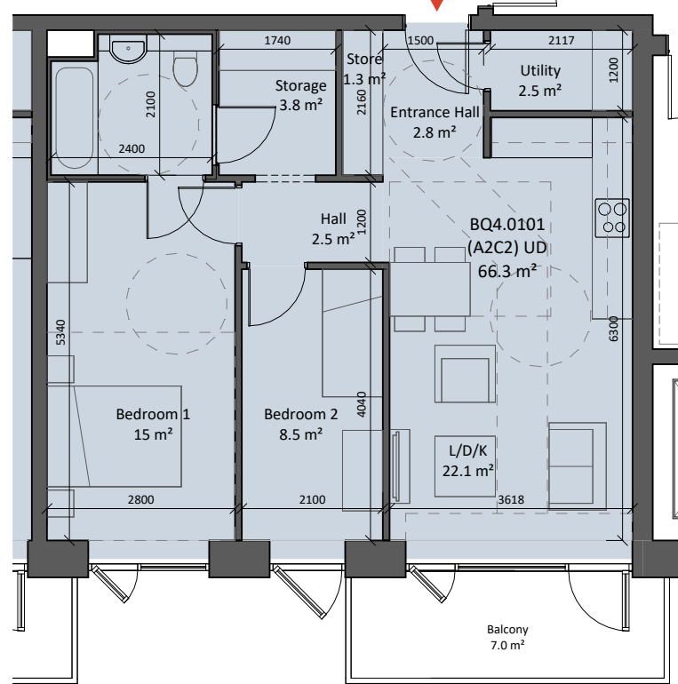
③ AT - A2C2 UD 1 : 100
