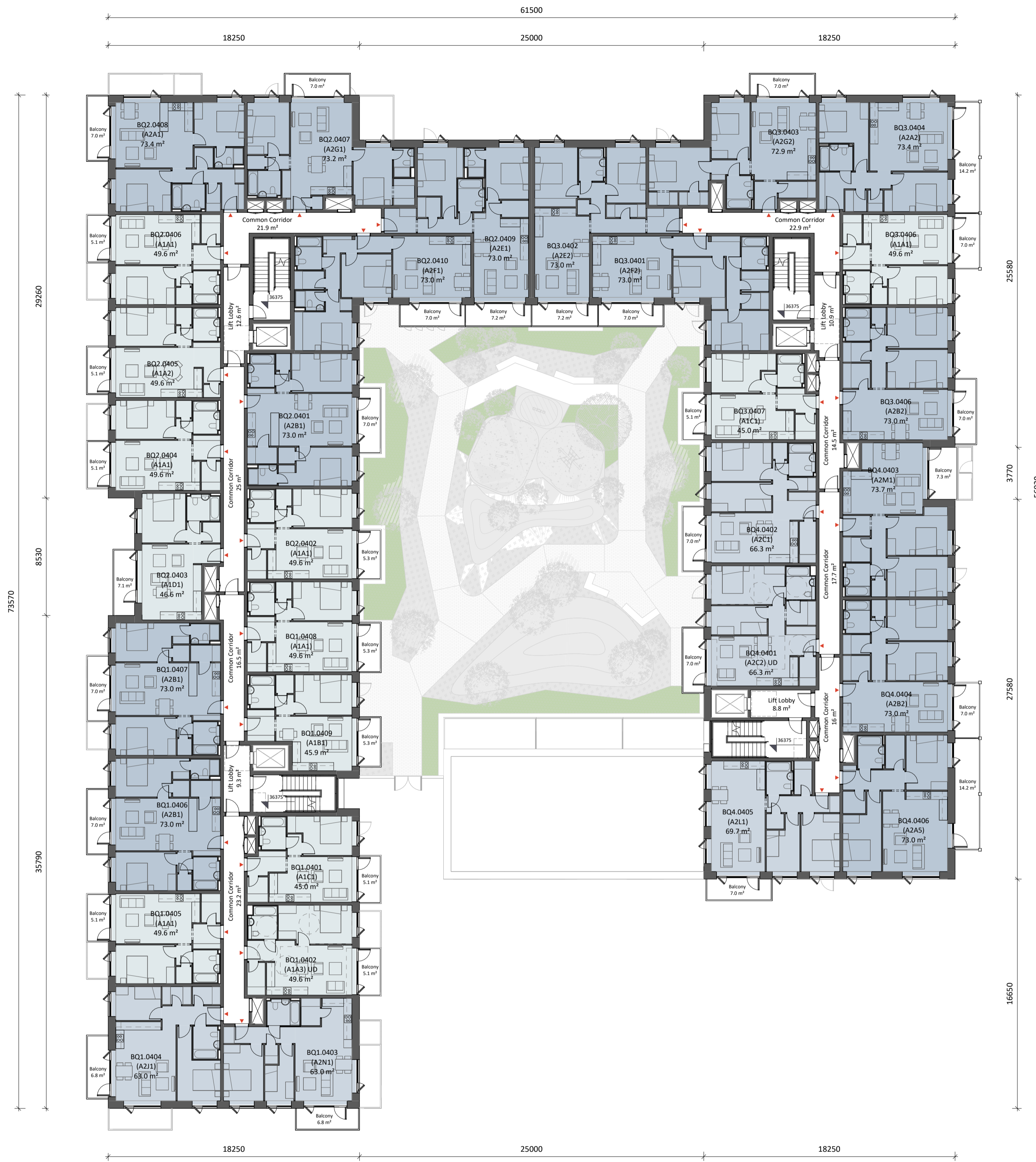
1 Block Q - Fourth Floor 1: 200
