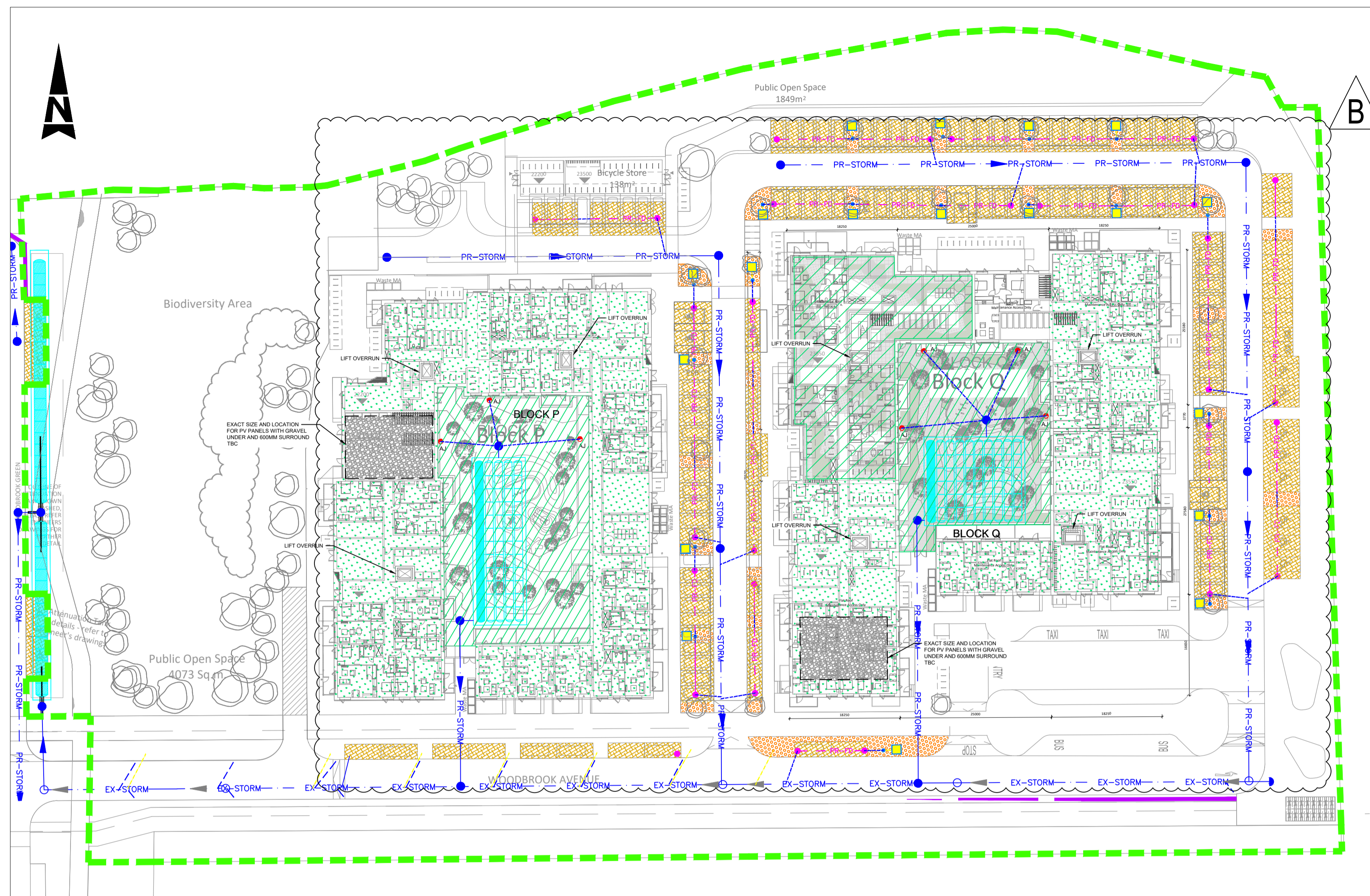
GREEN ROOF AREAS BLOCK P AND Q Scale at A1 1:500 at A1 Scale at A3 1:1000 at A3
