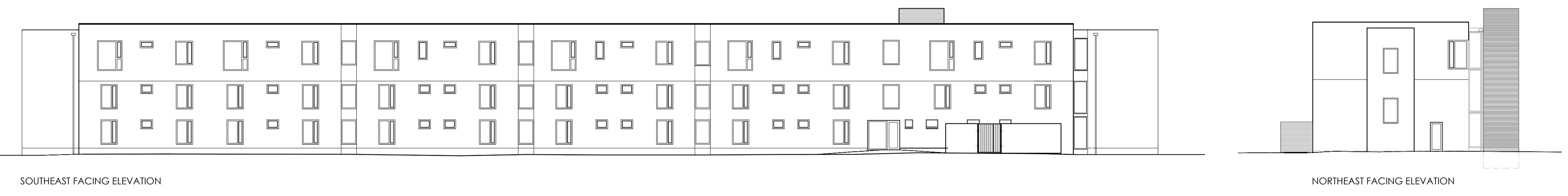
Existing Elevations Block 1 scale 1:200
