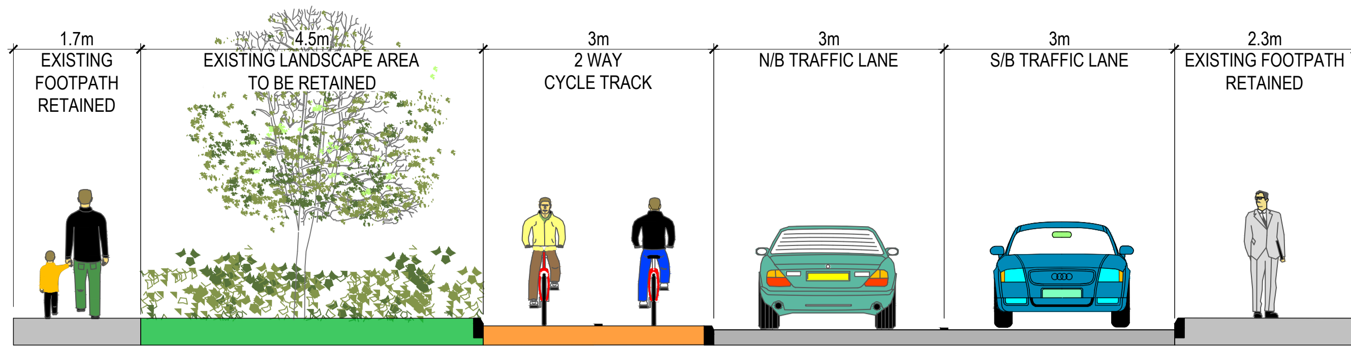
TYPICAL CROSS SECTION D-D SCALE 1:50
