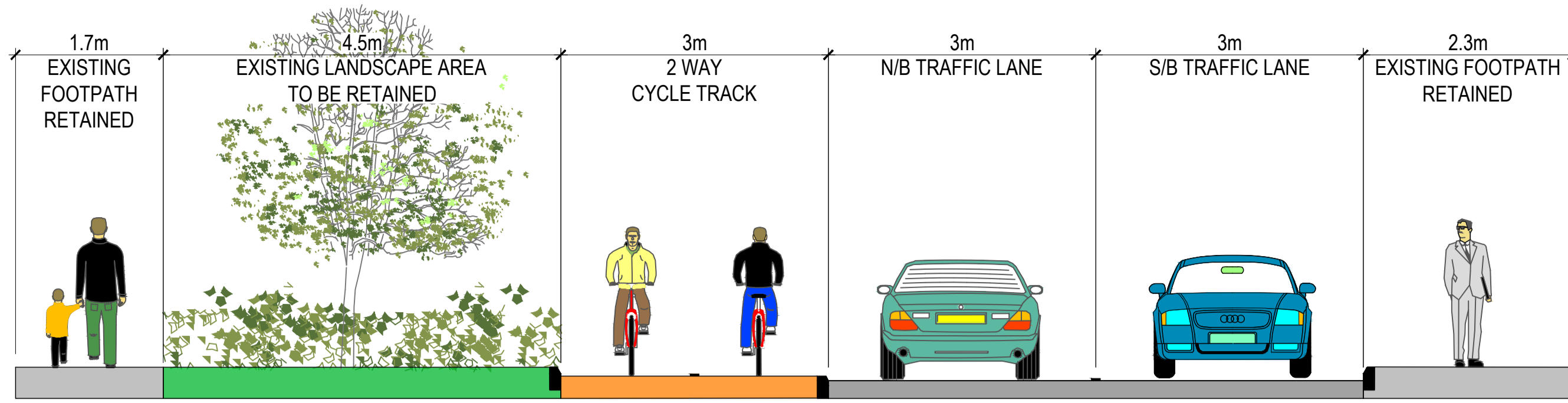
TYPICAL CROSS SECTION C-C SCALE 1:50
