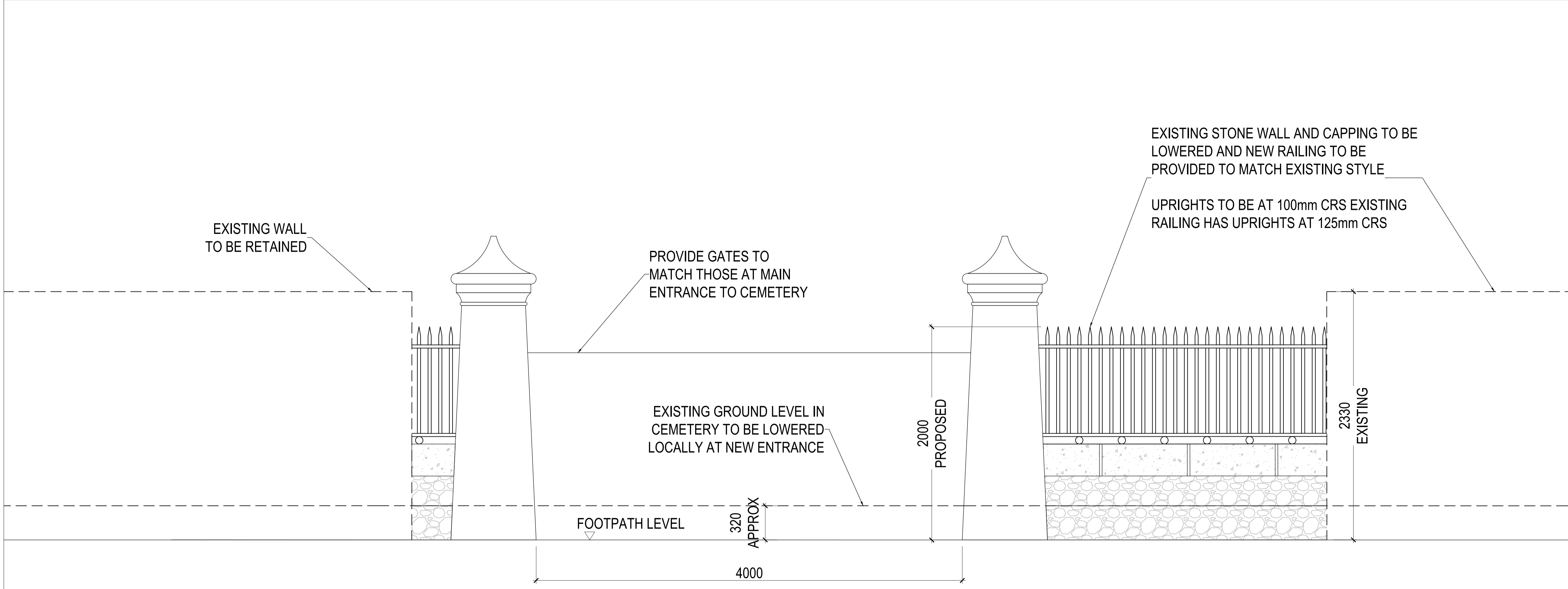
SECTION B-B SOUTHERN CEMETERY ENTRANCE SCALE 1:20
