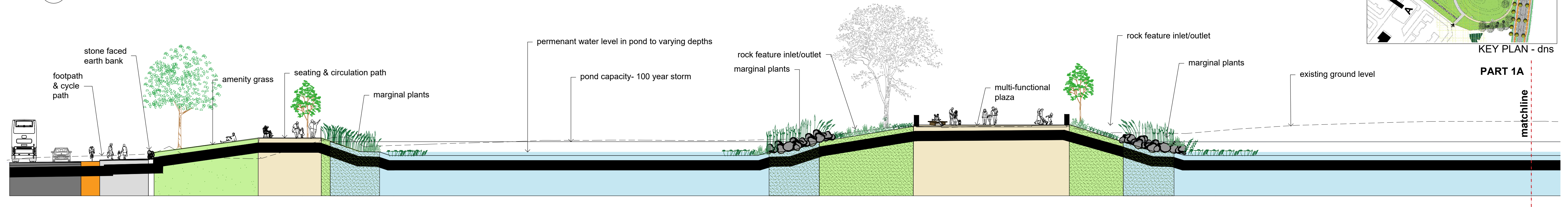
1A PART LANDSCAPE SECTION SCALE: 1:200@A1
