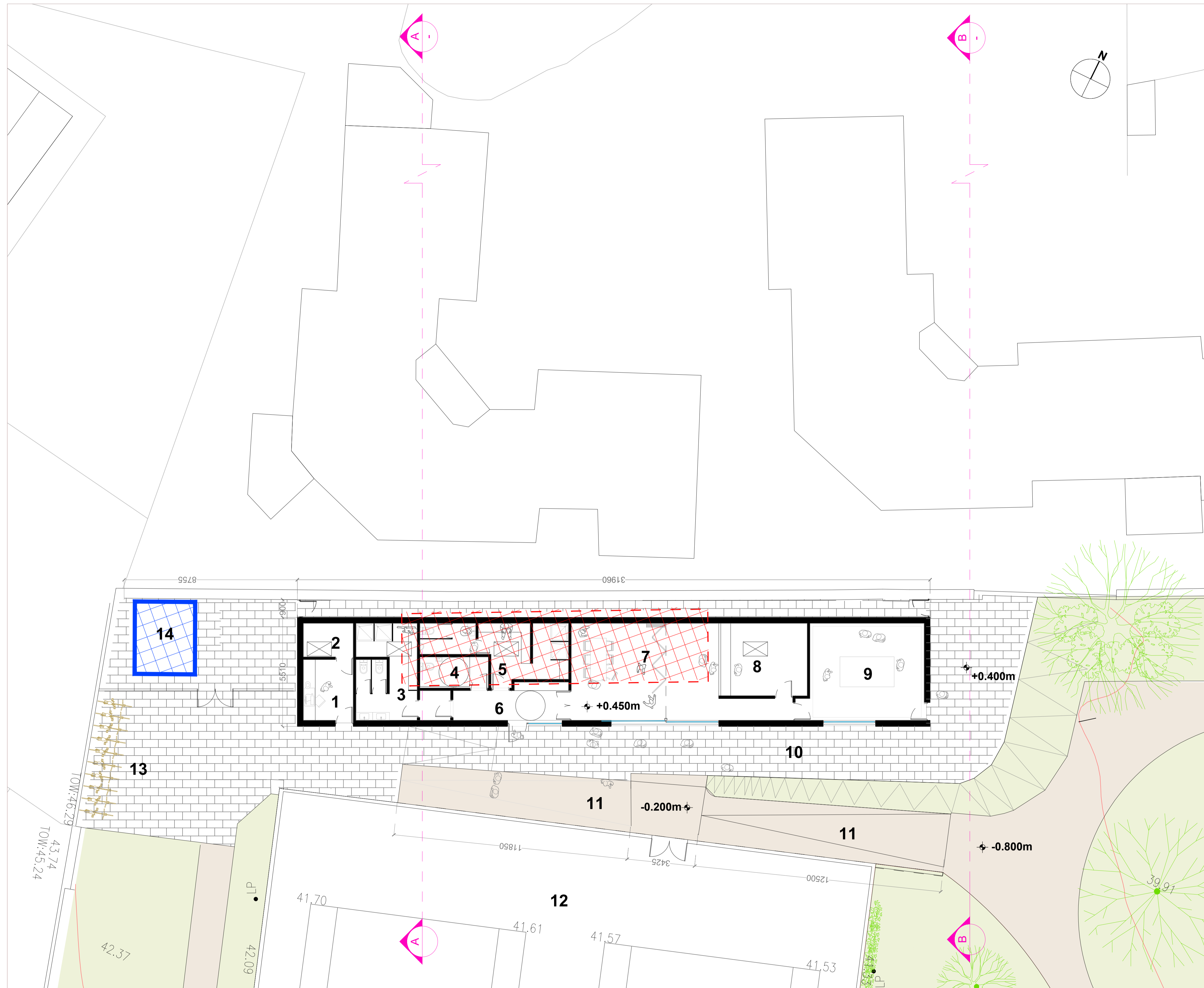
PROPOSED FLOOR PLAN (Scale - 1:100)
