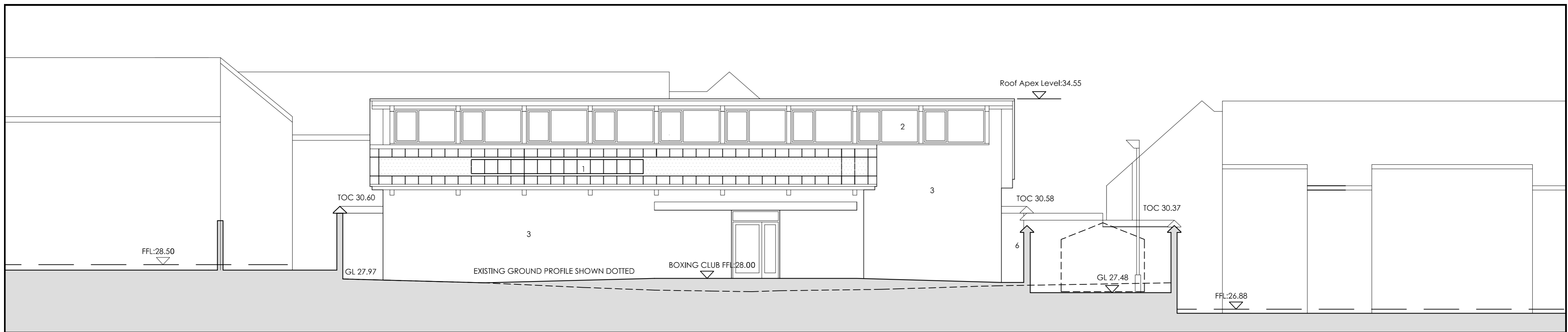
BOXING CLUB SITE 1105 1106 C-C SECTION / ELEVATION C-C
