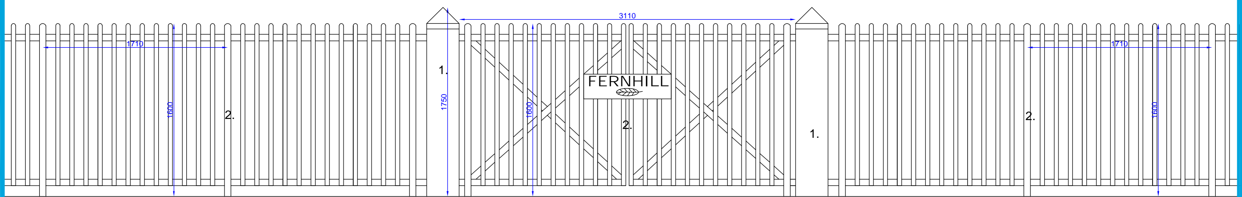
Indicative Detail 002: Gates & Railing at Belarmine
