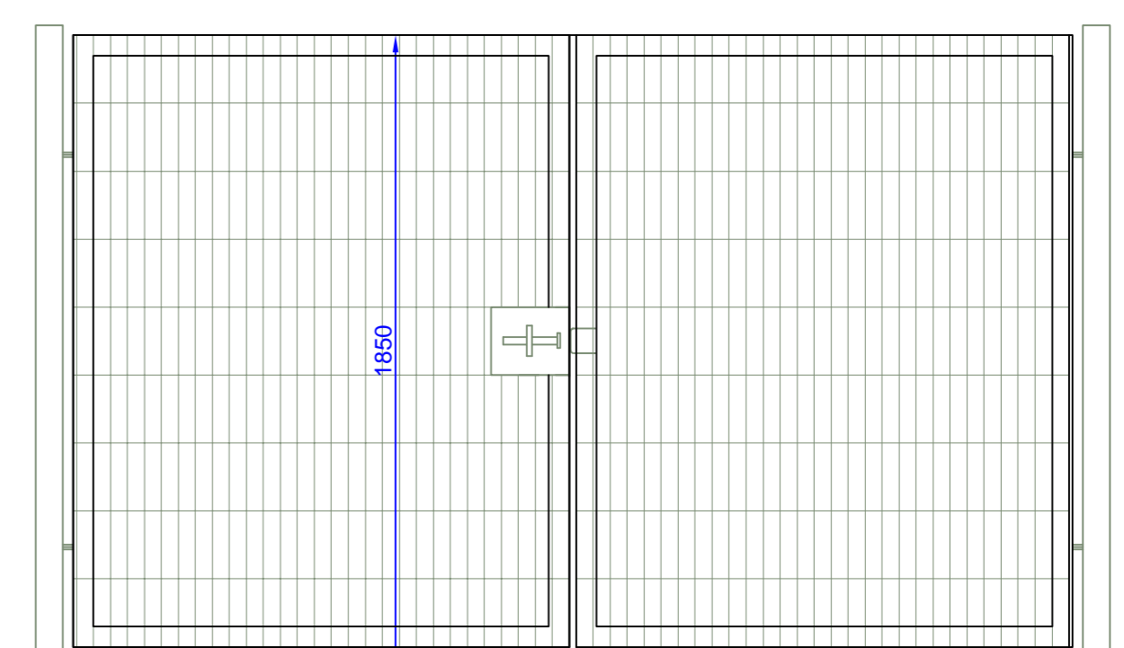
Indicative Detail 008: Right of Way Gate
