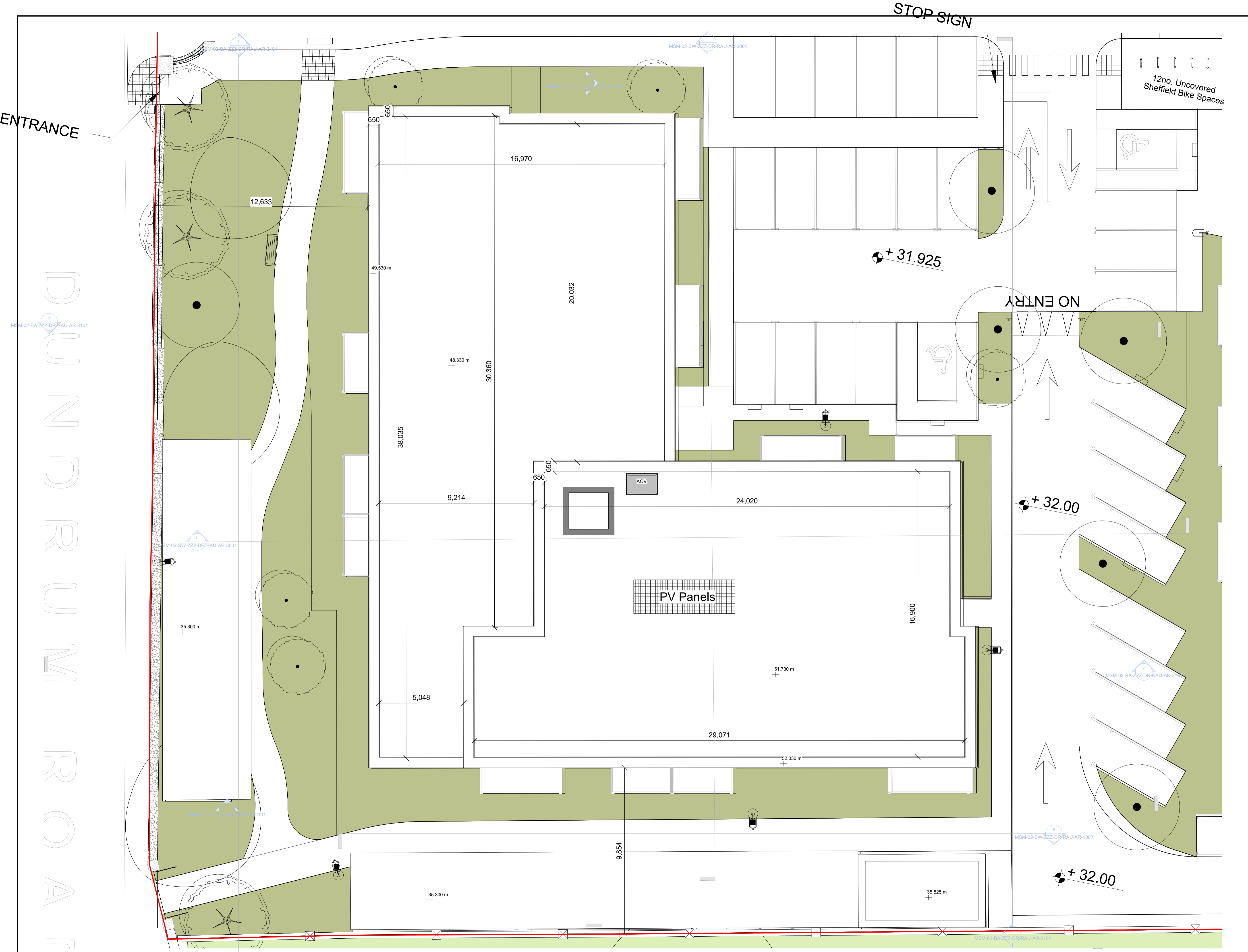
RF_Block A Roof Plan 1: 100
