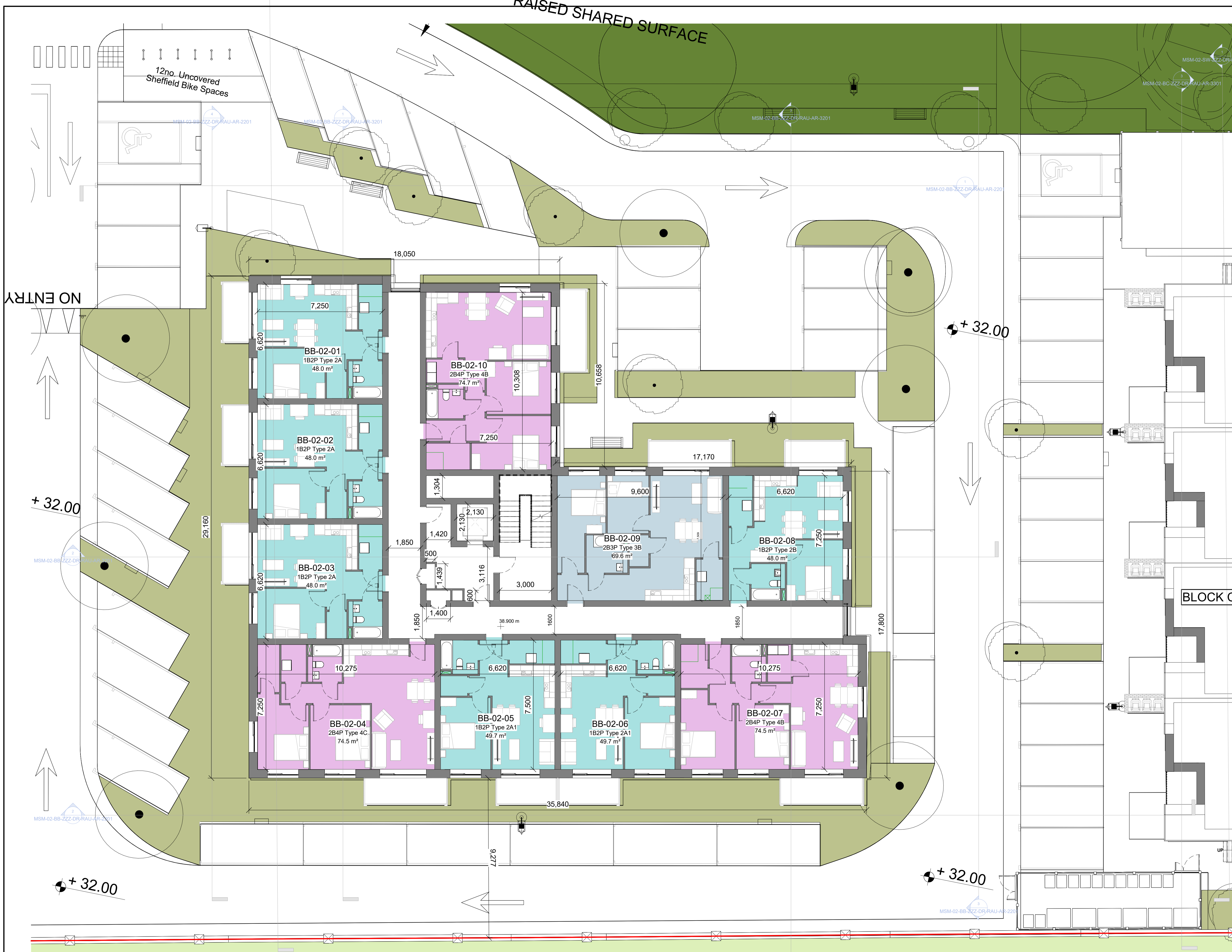
L02_Block B Second Floor Plan 1: 100
