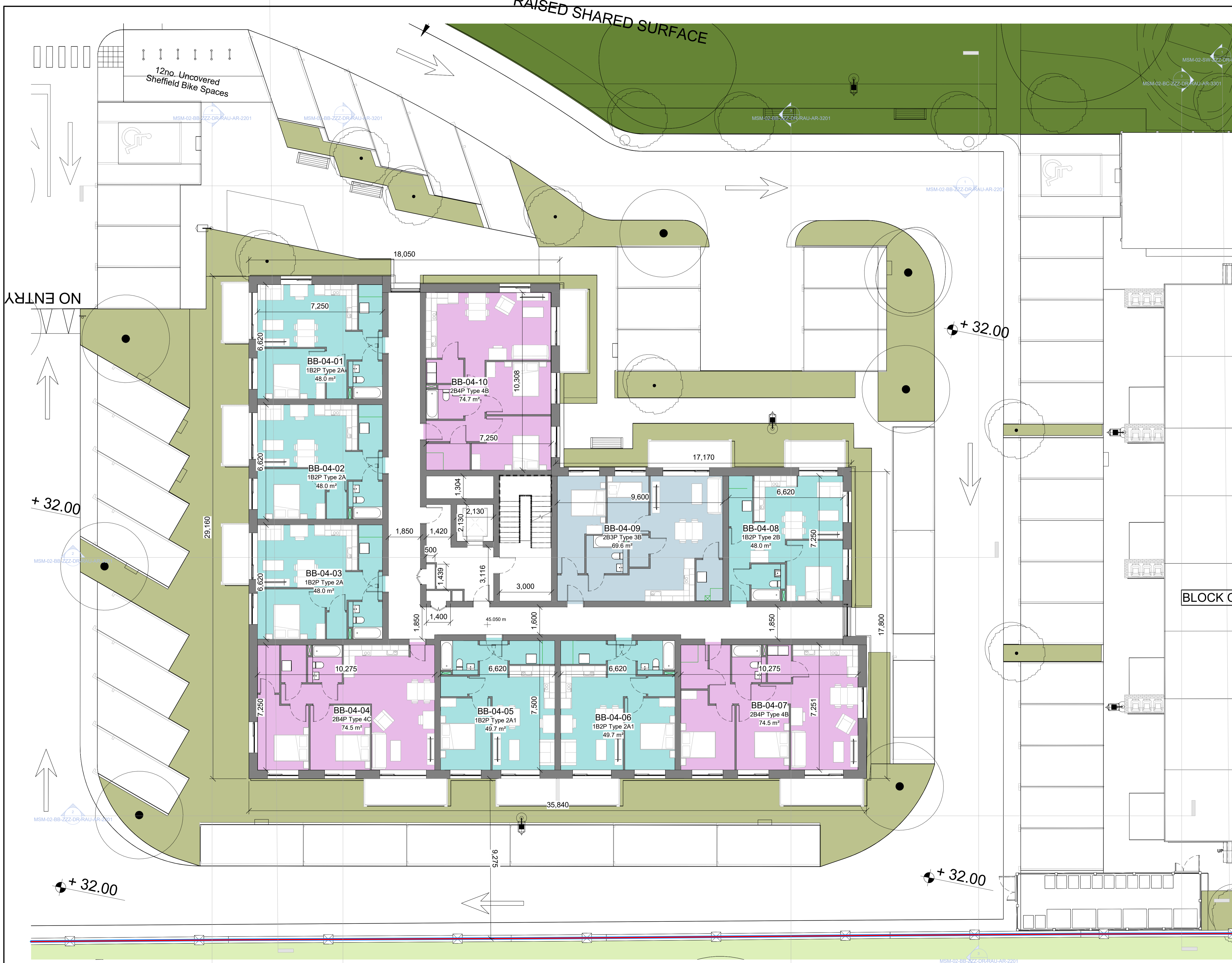
L04_Block B Fourth Floor Plan 1:100
