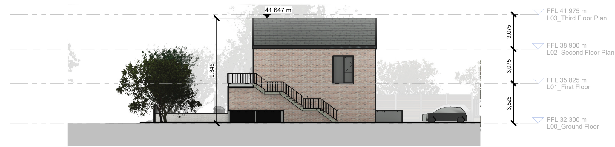
Block C, North Elevation 1 : 200
