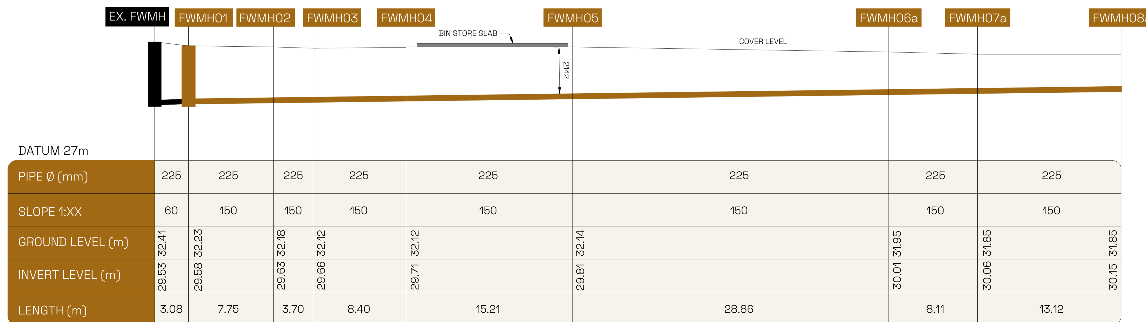
FW SECTION 2 SCALE 1:100 HORIZONTAL SCALE 1:200
