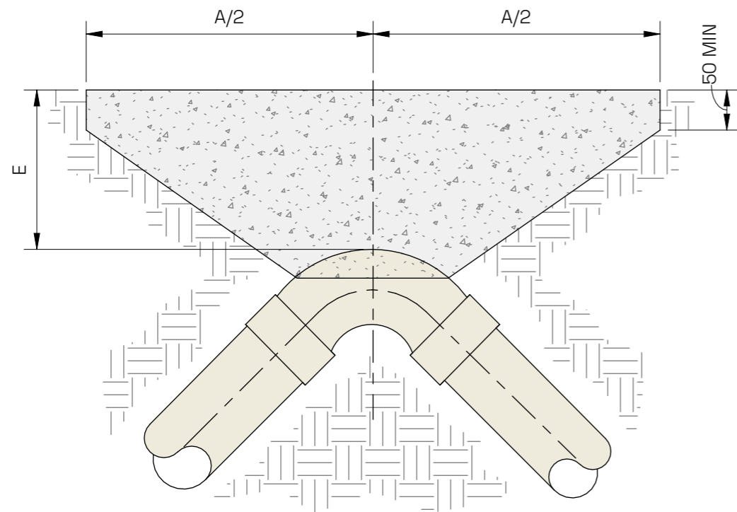
90 DEGREE BEND
