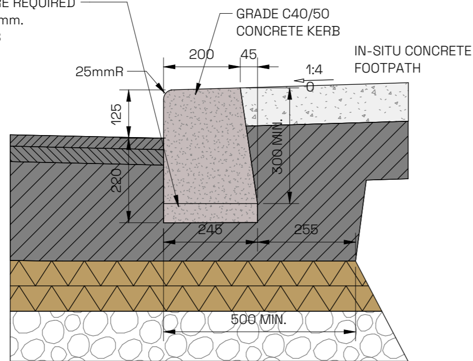
IN-SITU KERB WITH 250mm KERB SCALE 1:10 FACE
