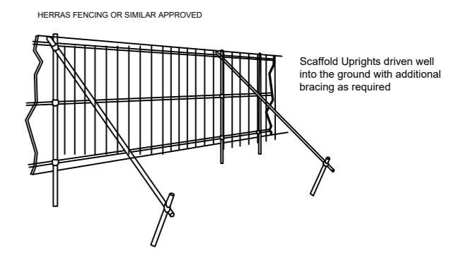
TREE PROTECTION DETAIL: HERRAS FENCING OR SIMILAR APPROVED
