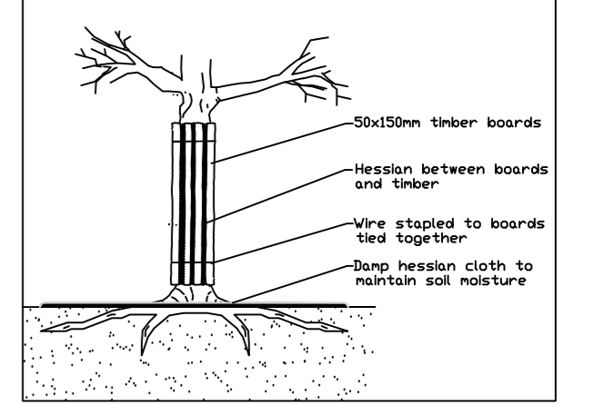
TIMBER BOARD TRUNK PROTECTION WHERE TREE PROTECTION FENCING CANNOT BE USED DUE TO SPACE RESTRICTIONS
