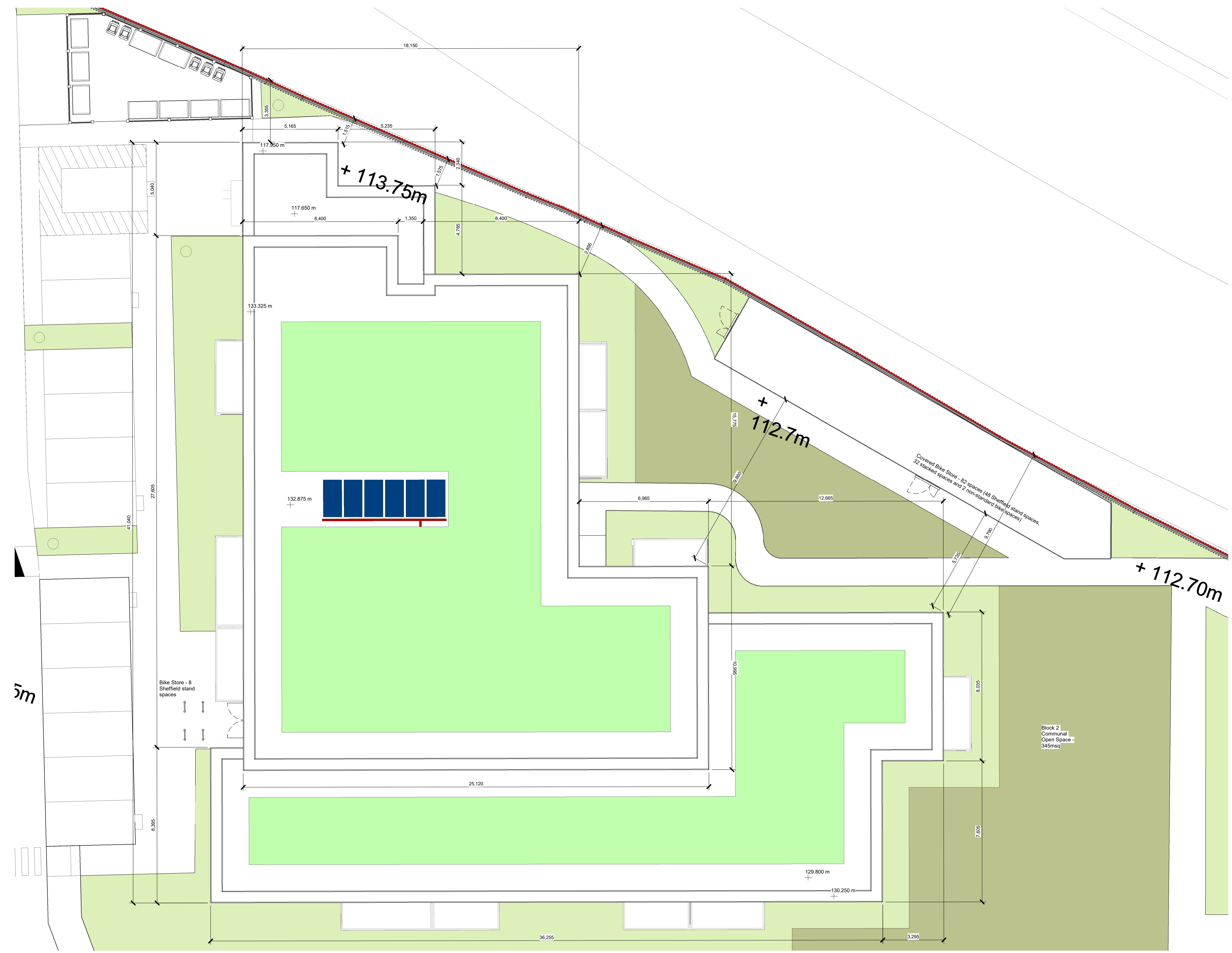
RF - Roof Level Apartment Block 1 : 100
