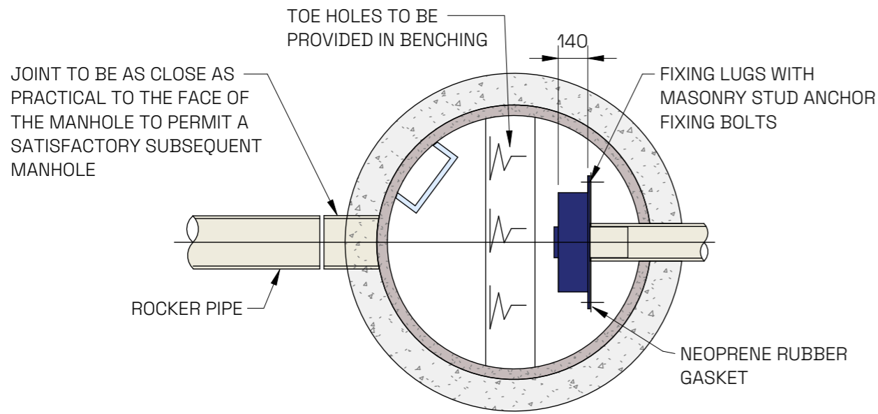
PLAN AT BENCHING LEVEL
