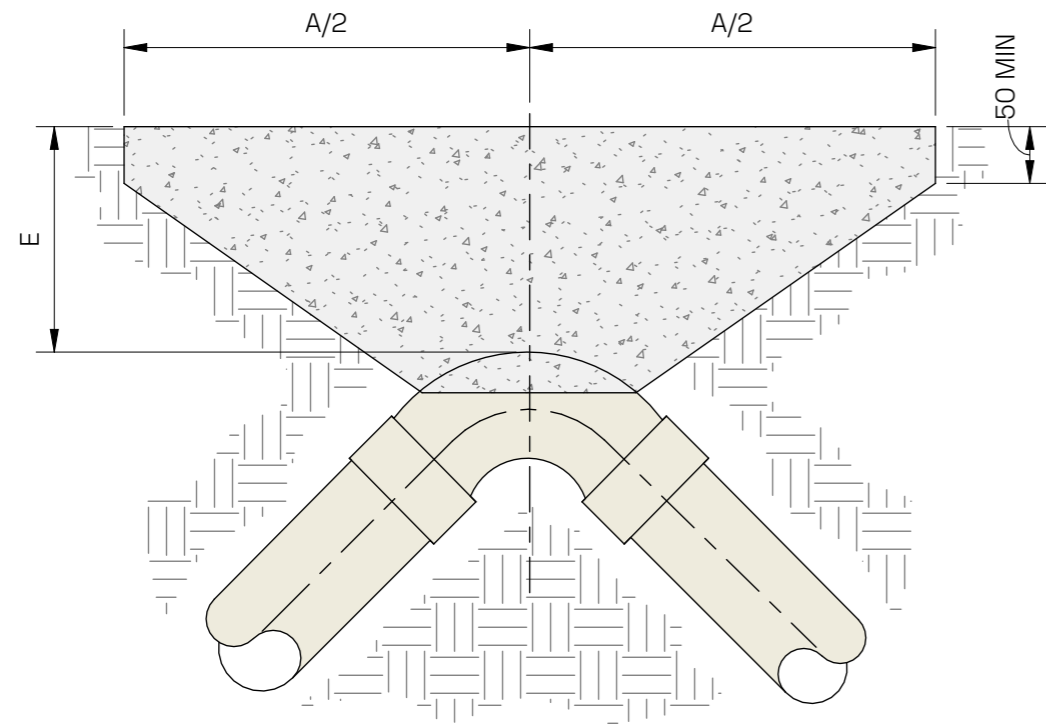
90 DEGREE BEND
