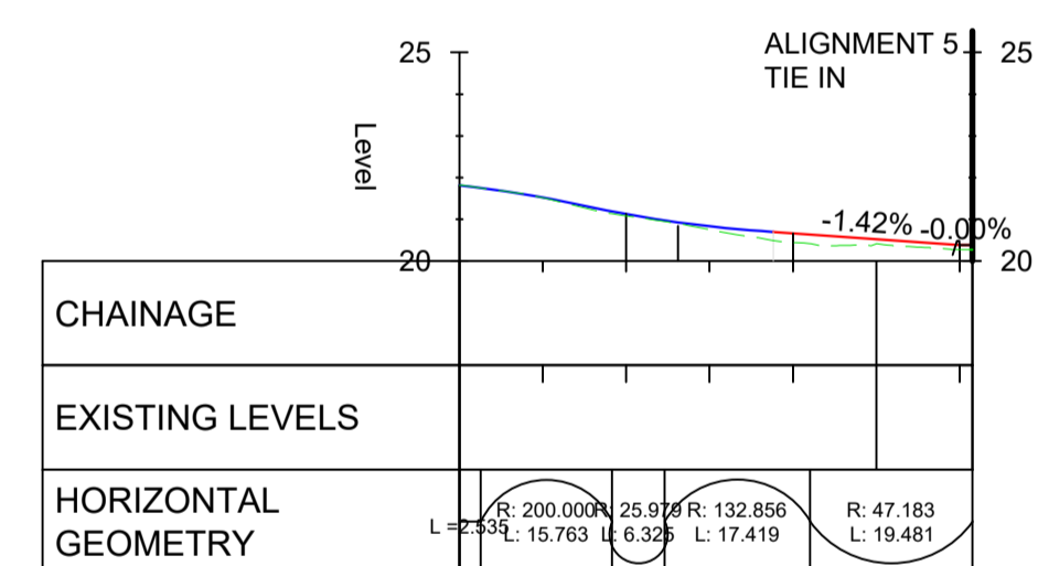
ALIGNMENT 13 - LONGSECTION SCALE: H 1:500,V 1:100. DATUM: 20.000
