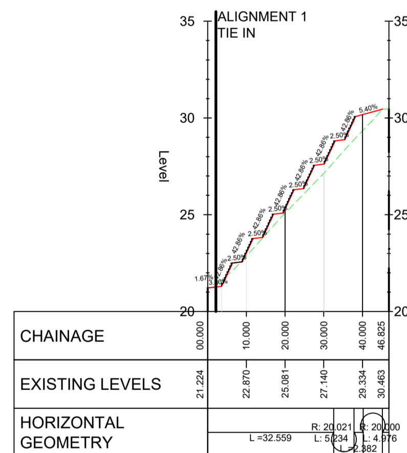
ALIGNMENT 12 - LONGSECTION SCALE: H 1:500,V 1:100. DATUM: 20.000
