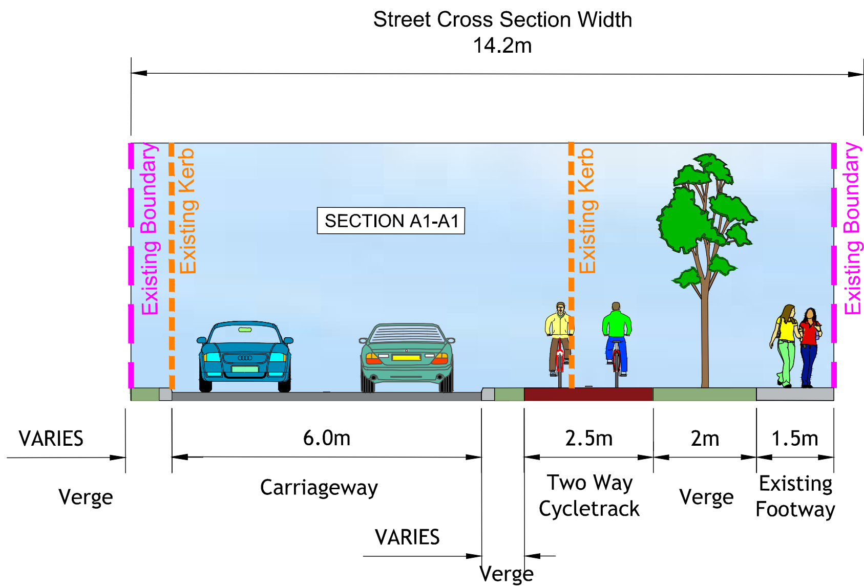
V3 - PROPOSED CROSS SECTION A1-A1 SCALE = 1:75
