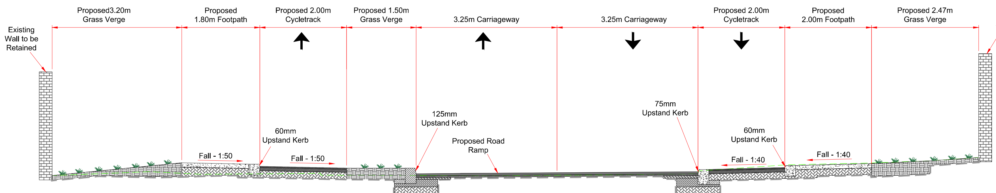
SECTION E-E SCALE - 1:50
