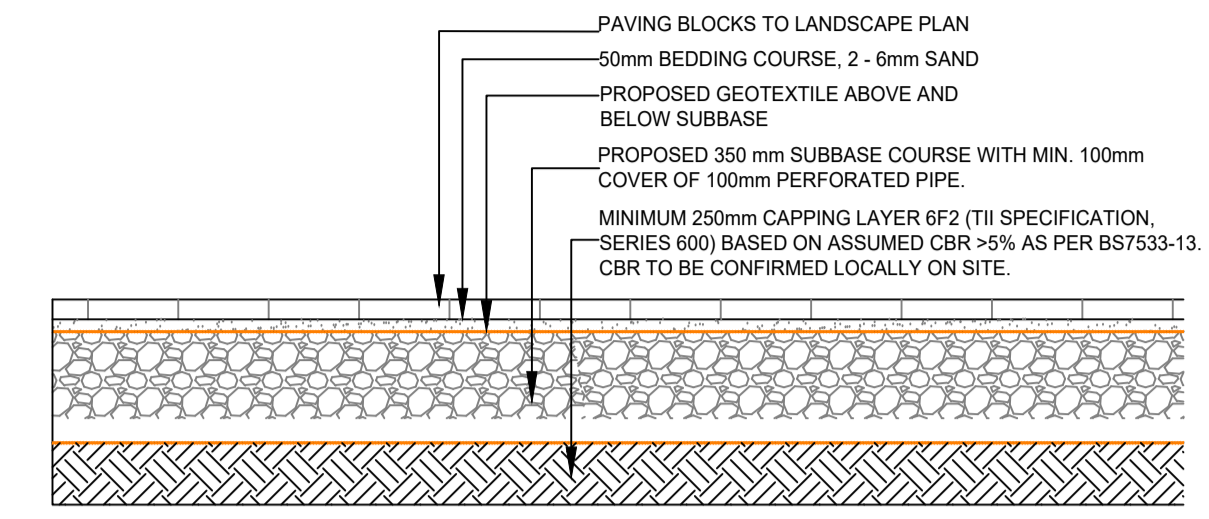
TYPICAL PERMEABLE PAVING BUILD-UP
